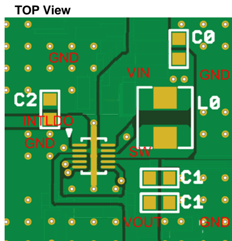
Figure 31. Reference Board Layout (TOP Layer)
