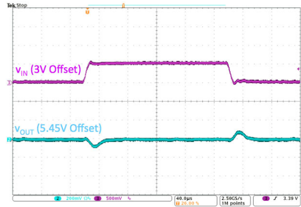
Figure 10. Line Transient, 3.0 V ↔ 3.5 V, 10 \mu\text{s} Edge, 550 mA Load
