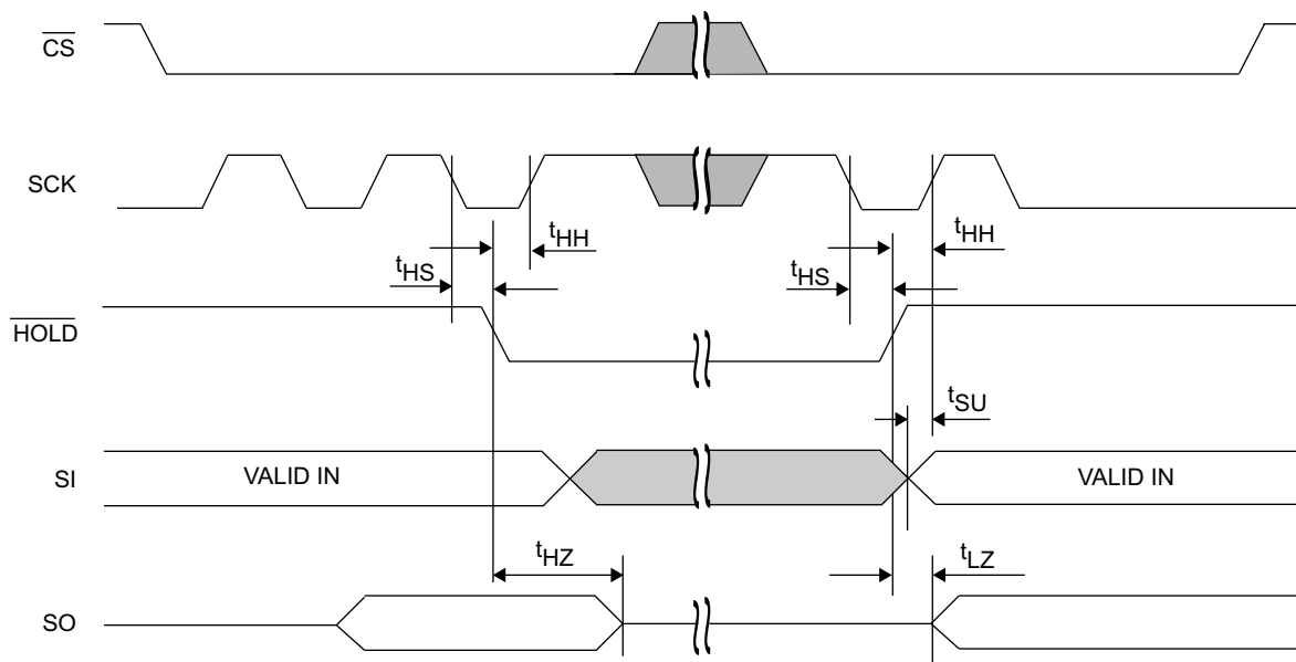
Figure 16. \overline{HOLD} Timing
