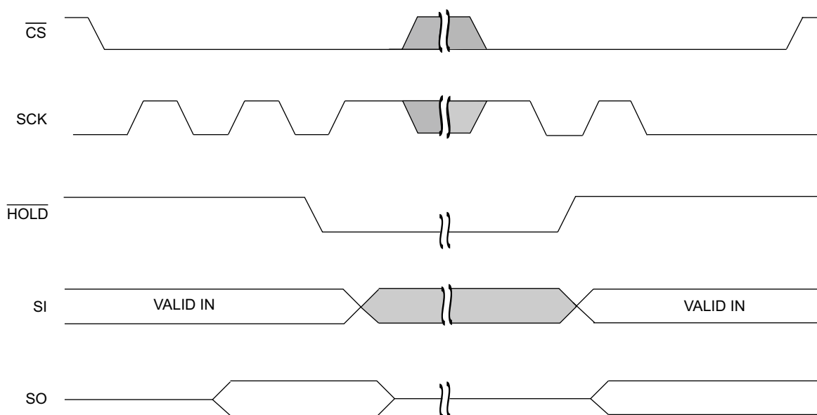
Figure 13. \overline{\text{HOLD}} Operation [2]
