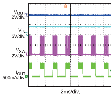
Short-Circuit Steady
