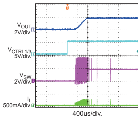
CTRL On
