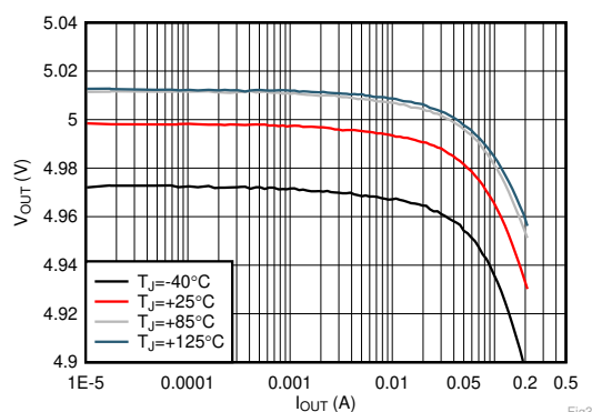
Load Regulation
