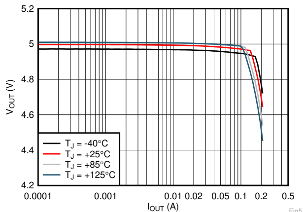
Figure 6-3. Load Regulation
