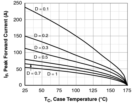
Figure 4. Current Derating
