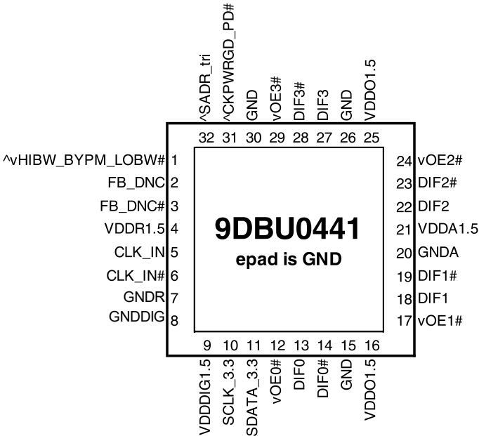
32-pin VFQFPN, 5x5 mm, 0.5mm pitch
