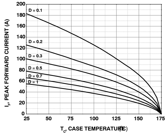
Figure 4. Current Derating
