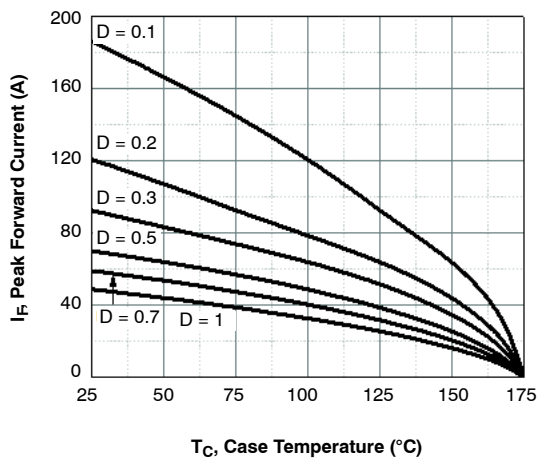
Figure 3. Current Derating
