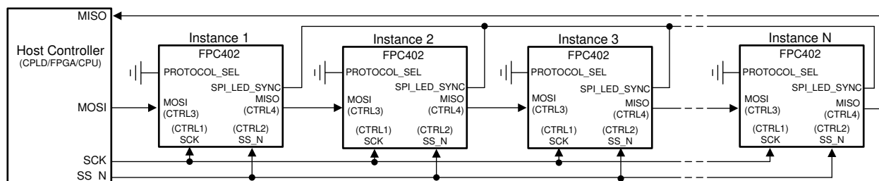
Figure 8-6. FPC402 Connection Diagram for SPI Mode
