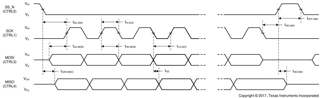
Figure 8-9. SPI Timing Diagram
