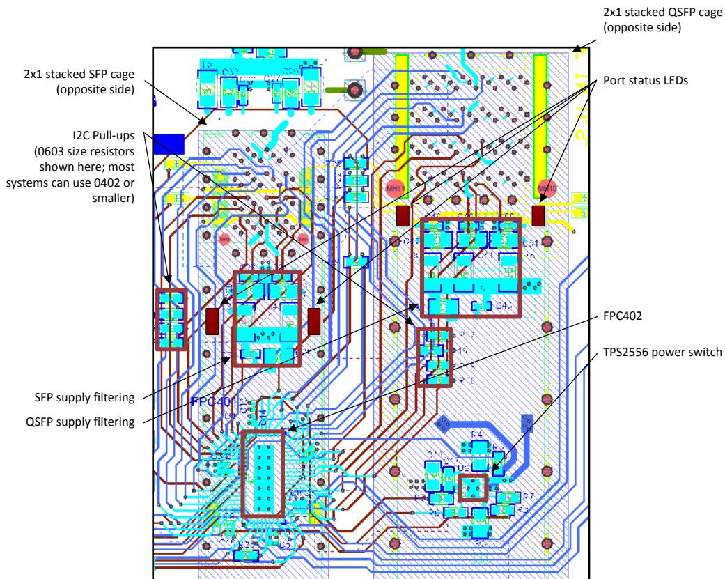
Figure 11-1. Layout Example
