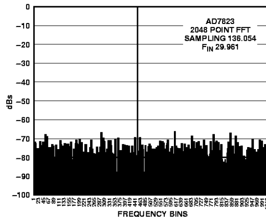
Figure 3. AD7823 SNR
