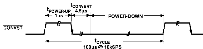
Figure 13. Automatic Power-Down
