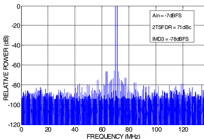
FIGURE 16. TWO-TONE SPECTRUM; f_{\text{IN}} = 69\text{MHz}, 70\text{MHz}
