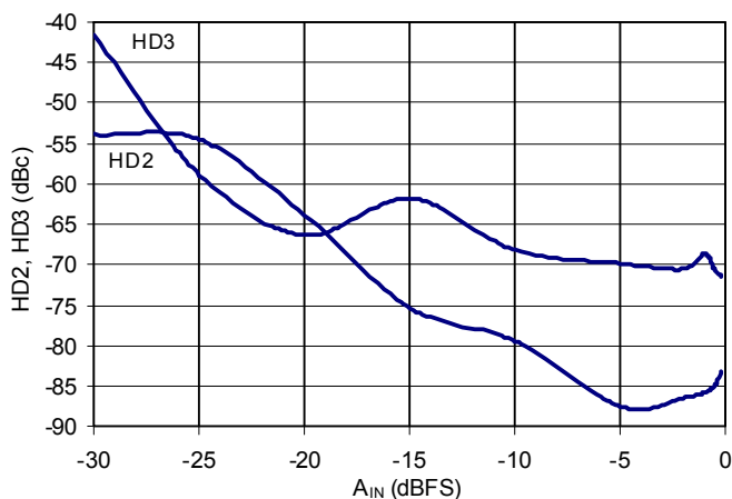
FIGURE 6. HD2 AND HD3 vs A_{\text{IN}}
