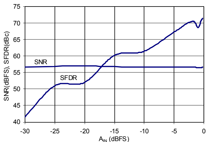
FIGURE 5. SNR AND SFDR vs A_{\text{IN}}
