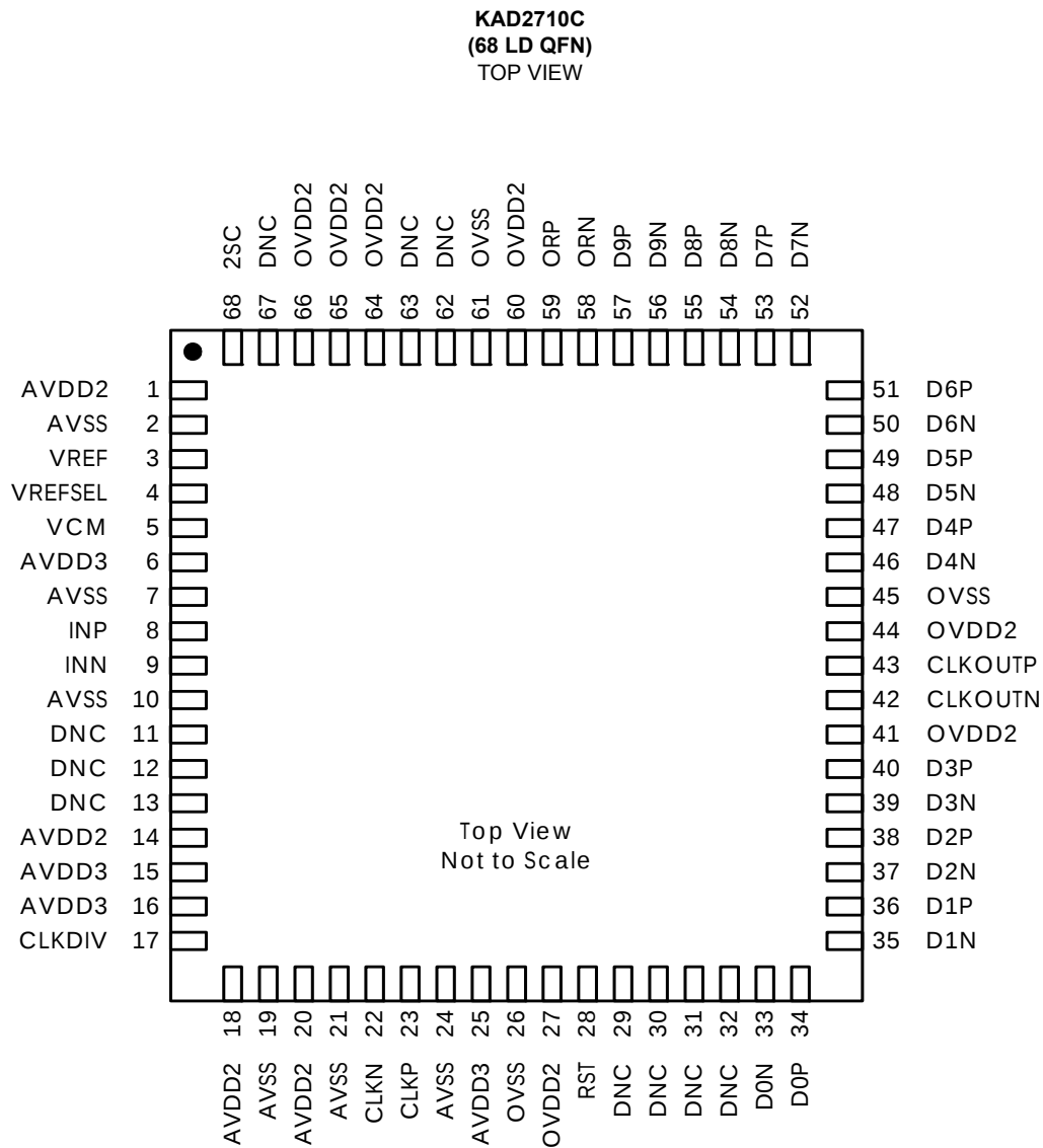
FIGURE 2. PIN CONFIGURATION
