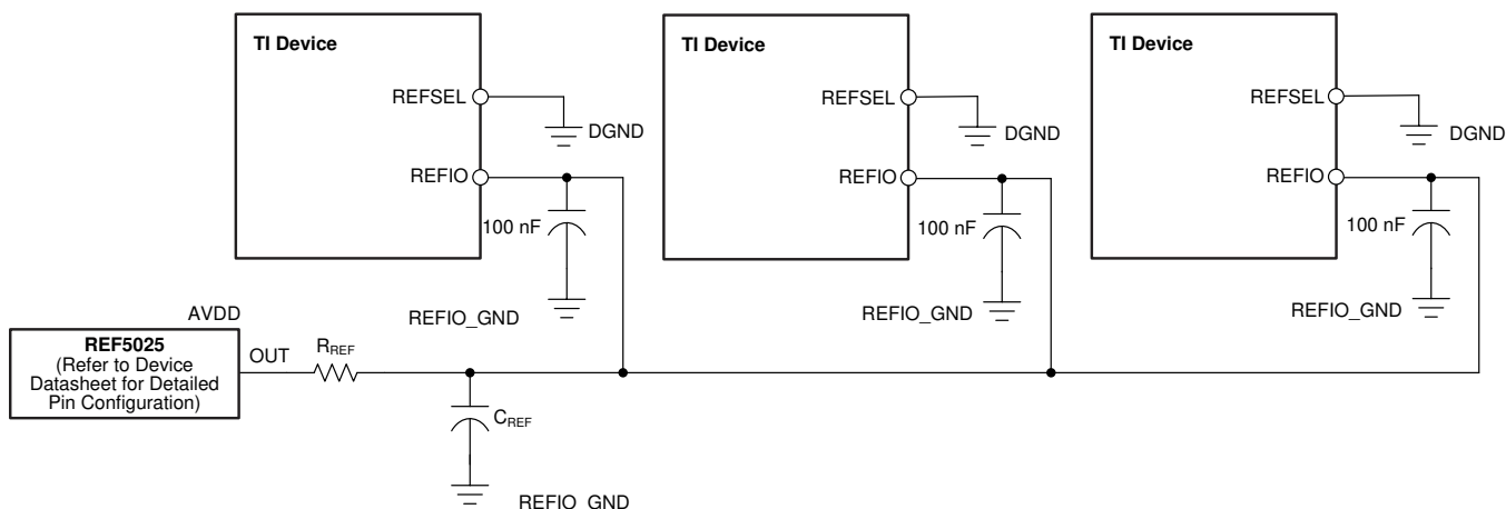
Figure 53. Multiple Devices Connected Using an External Reference
