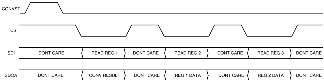
Figure 76. Serial Interface Register Read
