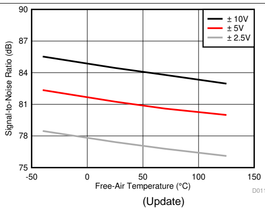
Figure 16. SNR vs Free-Air Temperature (Filter Option 3)
