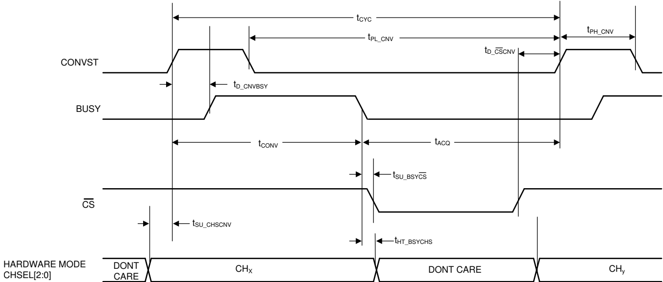
Figure 1. Universal Timing Diagram Across All Interfaces
