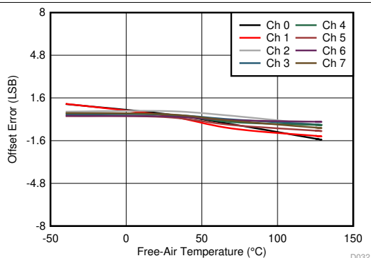
Figure 36. Offset Error vs Free-Air Temperature ( \pm 10\text{ V} , Across Channels)
