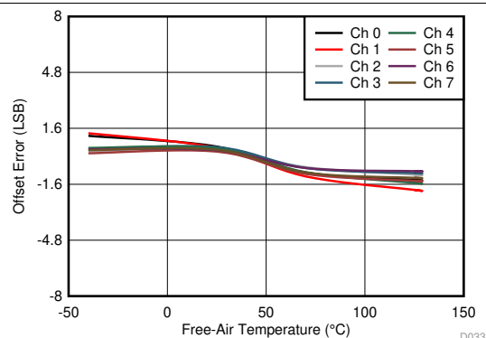
Figure 37. Offset Error vs Free-Air Temperature ( \pm 5\text{ V} , Across Channels)
