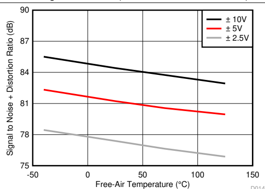
Figure 19. SINAD vs Free-Air Temperature (Filter Option 3)
