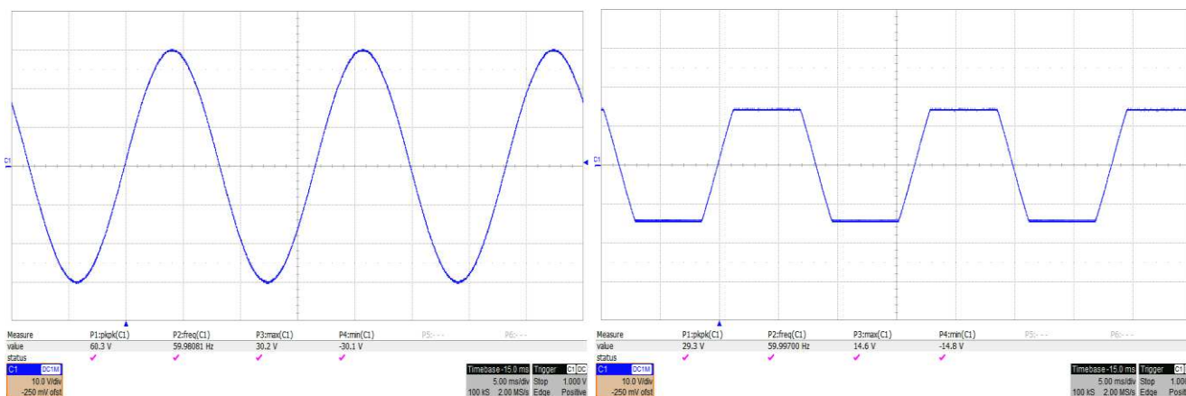
Figure 124. Input Protection Response Using a PTC Diode, a TVS Diode, and the ADS8686S
