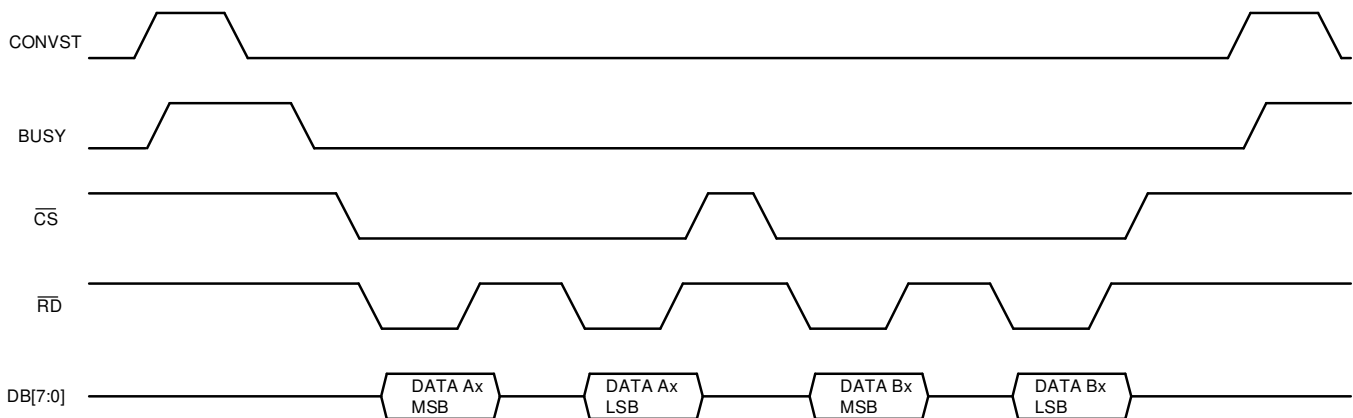
Figure 70. Parallel Byte Interface Conversion Readback
