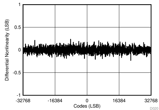
Figure 25. Typical DNL for All Codes ( \pm 10\text{ V} )
