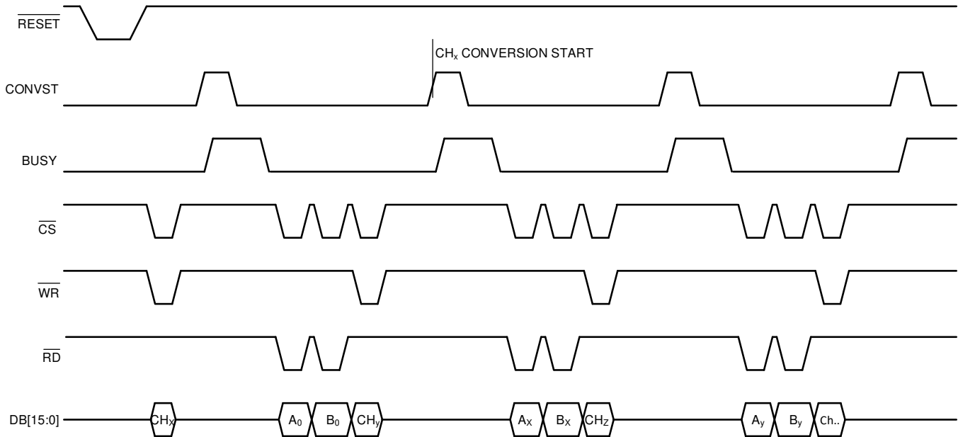
Figure 59. Software Parallel Mode Channel Conversion Setting
