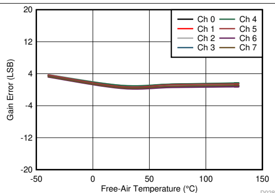
Figure 31. Gain Error vs Free-Air Temperature ( \pm 10\text{ V} , Across Channels)
