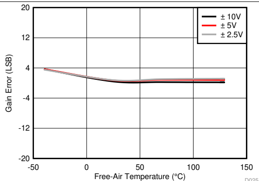
Figure 30. Gain Error vs Free-Air Temperature
