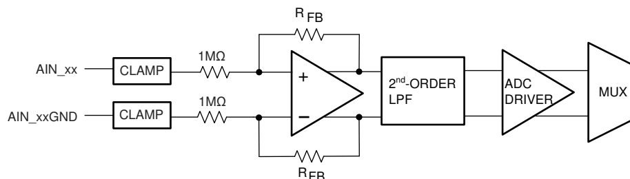
Figure 46. Analog Input Circuitry
