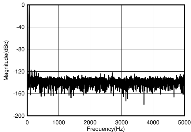
Figure 122. Captured Frequency Spectrum
