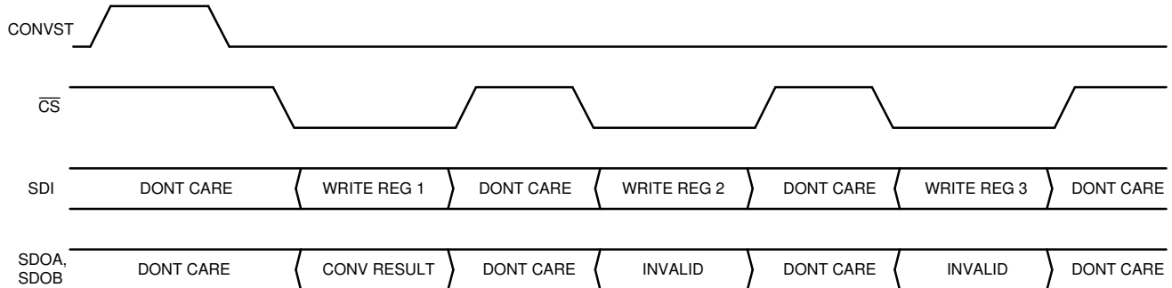
Figure 75. Serial Interface Register Write
