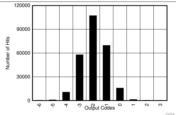
Figure 27. Typical Offset Error Histogram ( \pm 10\text{ V} )
