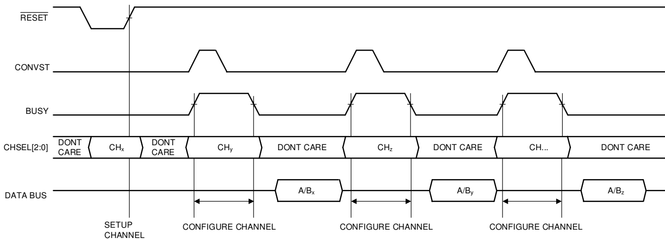
Figure 56. Hardware Mode Channel Conversion Setting
