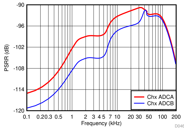
Figure 125. PSRR Across Frequency
