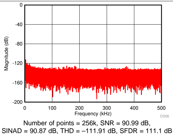
Figure 11. Typical FFT Plot ( \pm 5\text{ V} , Normal Mode, Filter Option 2)
