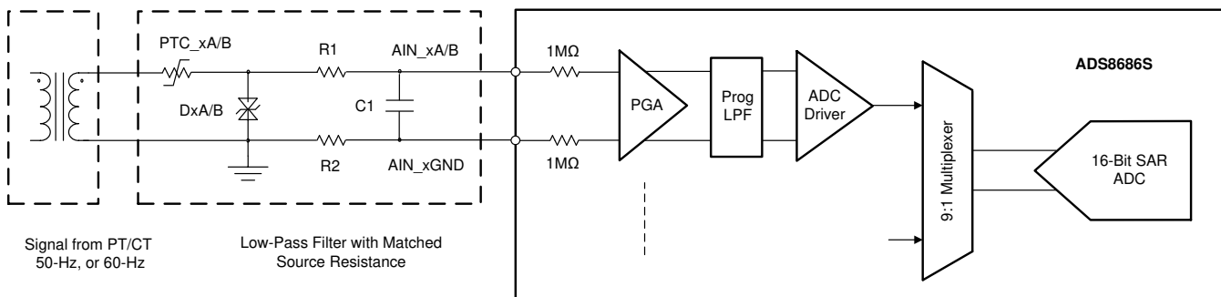
Figure 123. Input Protection for Electrical Overstress
