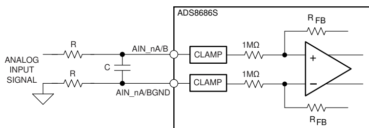
Figure 48. Input Resistance Matching on the Analog Input
