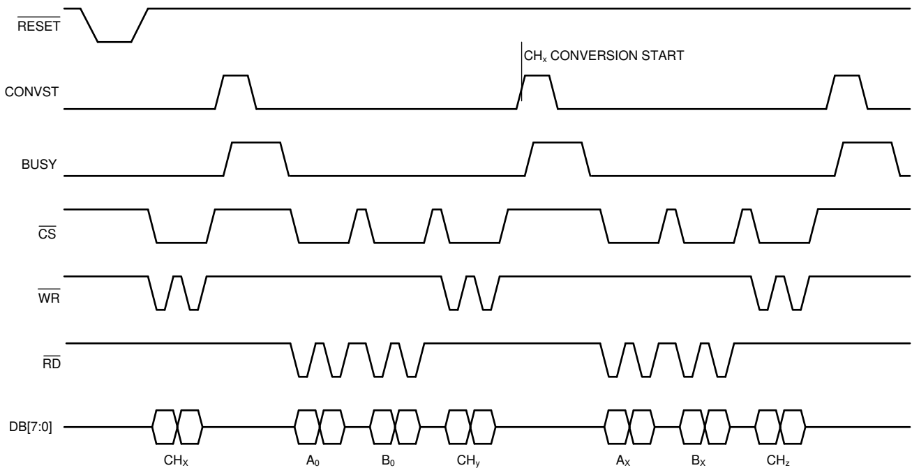
Figure 58. Software Parallel Byte Mode Channel Conversion Setting
