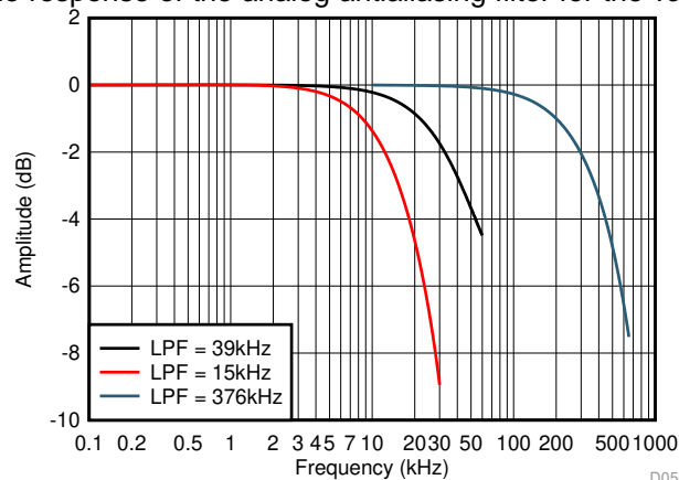
Figure 49. Second-Order LPF Magnitude Response
