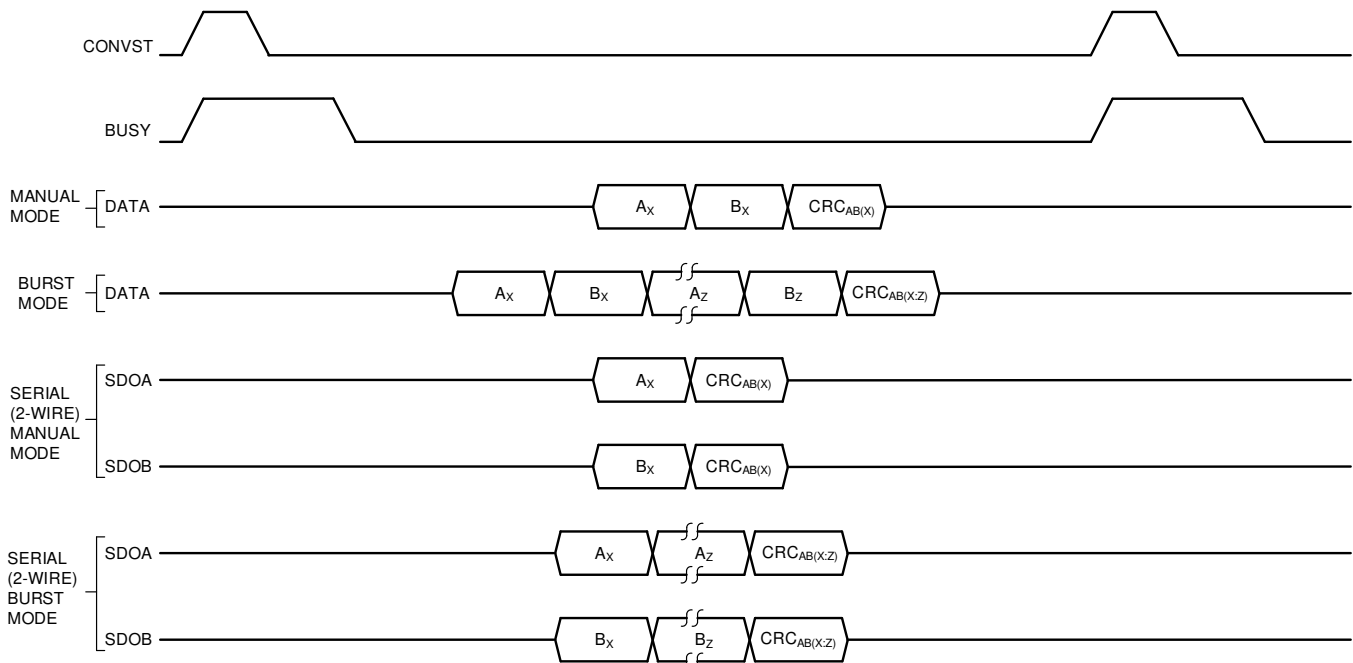
Figure 66. CRC Readback for All Modes
