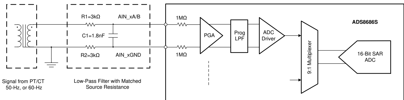
Figure 121. Input RC Low-Pass Filter
