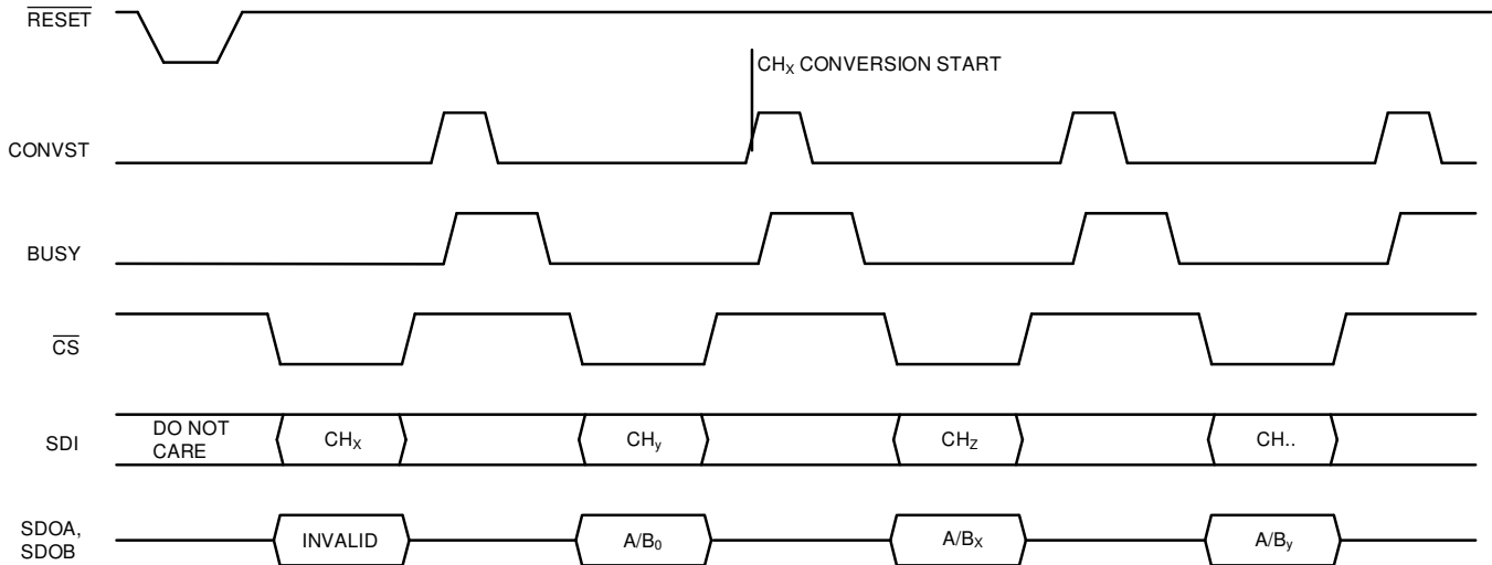
Figure 57. Software Serial Mode Channel Conversion Setting
