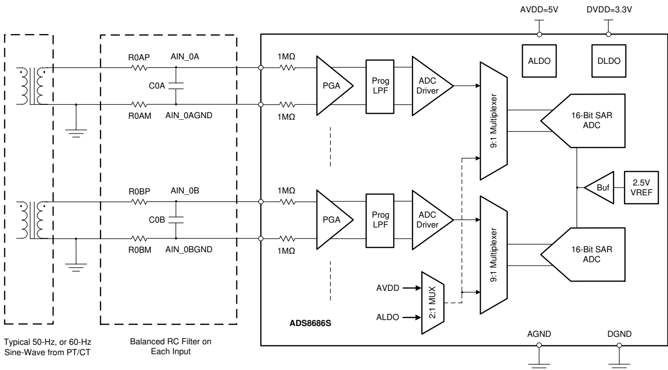
Figure 120. DAQ for Power Automation Using the ADS8686S
