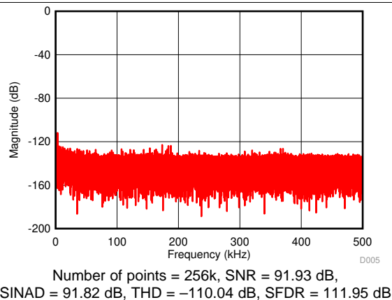
Figure 10. Typical FFT Plot ( \pm 10\text{ V} , Normal Mode, Filter Option 2)
