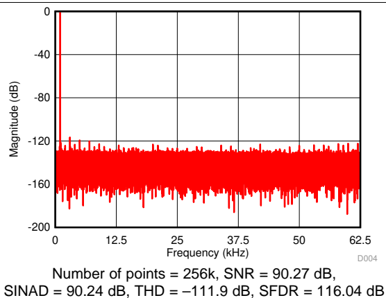
Figure 9. Typical FFT Plot ( \pm 10\text{ V} , Burst Mode, Filter Option 1)
