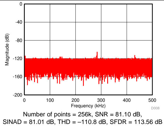
Figure 13. Typical FFT Plot ( \pm 5\text{ V} , Normal Mode, Filter Option 3)
