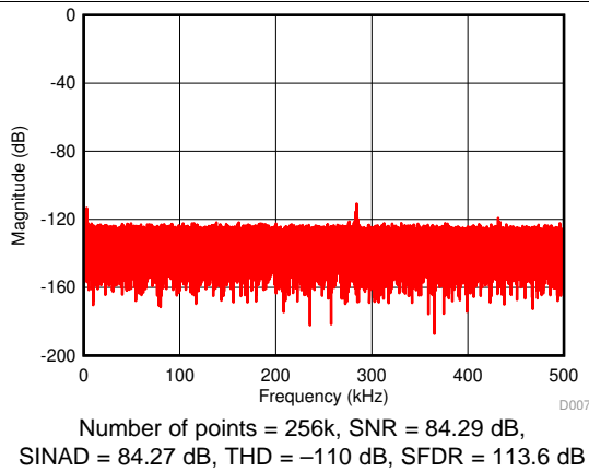
Figure 12. Typical FFT Plot ( \pm 10\text{ V} , Normal Mode, Filter Option 3)
