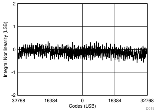
Figure 24. Typical INL for All Codes ( \pm 5\text{ V} )
