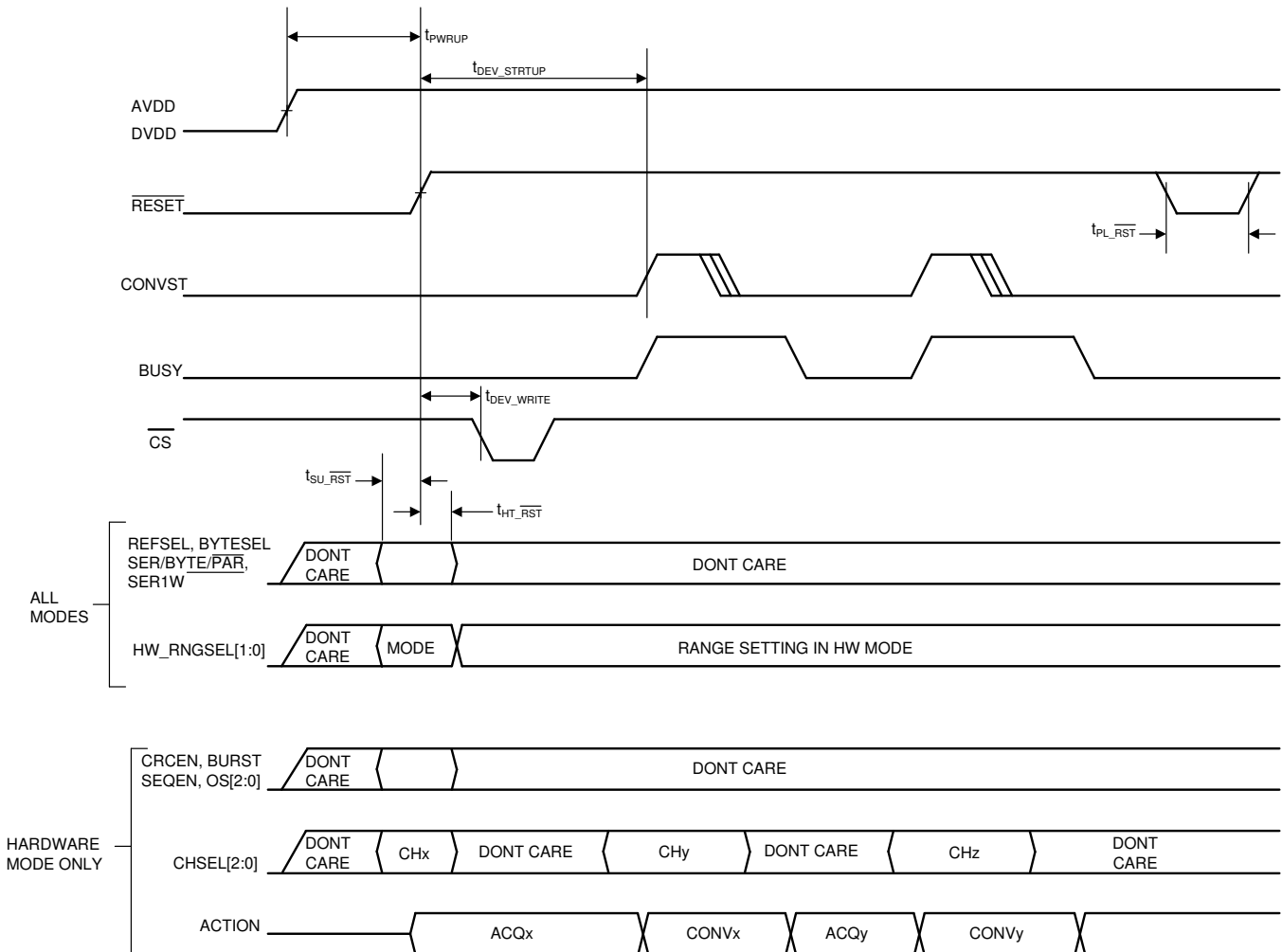
Figure 55. ADS8686S Configuration at Reset
