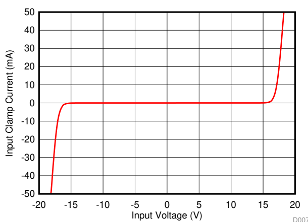
Figure 47. Input Protection Clamp Profile, Input Clamp Current vs Source Voltage
