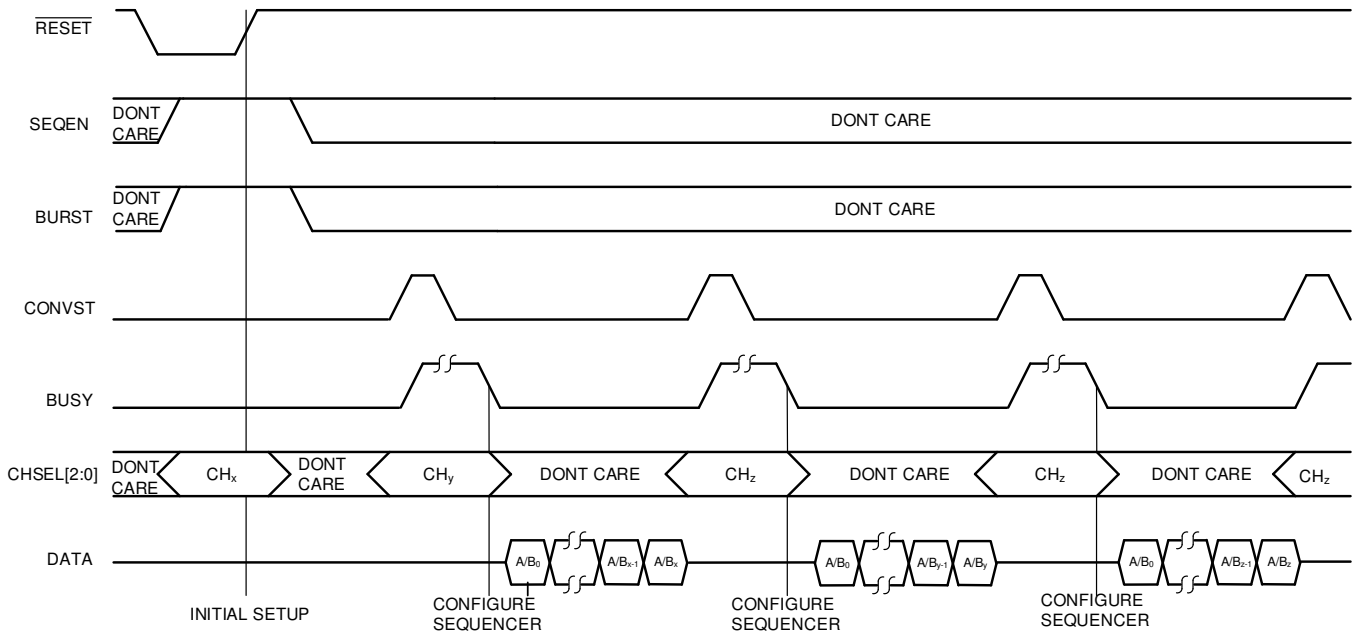
Figure 62. Burst Sequencer, Hardware Mode
