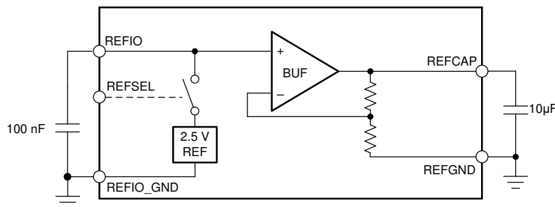
Figure 50. Reference Circuitry
