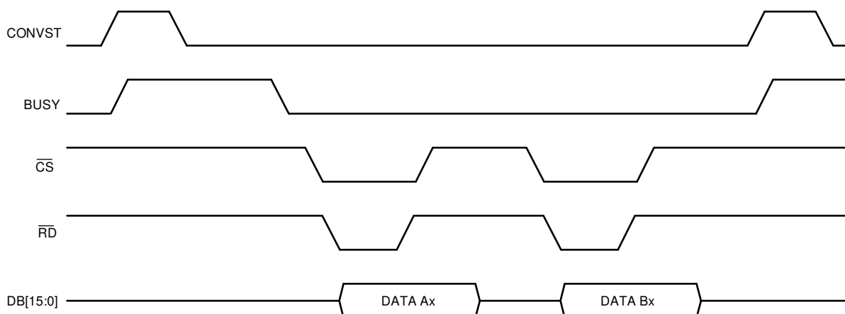
Figure 67. Parallel Interface Conversion Readback
