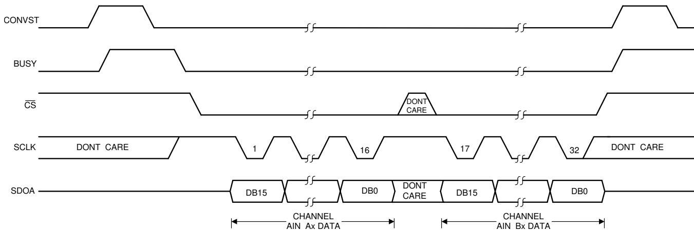
Figure 74. Serial Interface, 1-Wire Mode
