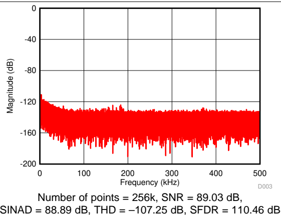
Figure 8. Typical FFT Plot ( \pm 2.5\text{ V} , Normal Mode, Filter Option 1)
