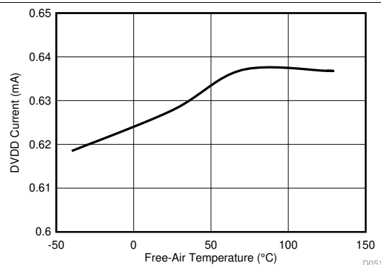
Figure 41. DVDD Current vs Free-Air Temperature
