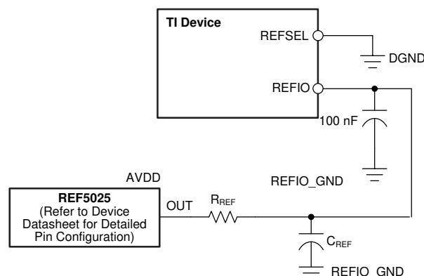
Figure 51. Device Connections for Using an External 2.5-V Reference
