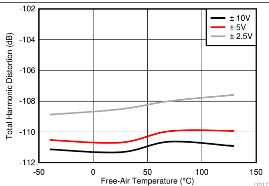
Figure 20. THD vs Free-Air Temperature (Filter Option 1)
