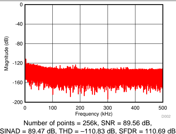
Figure 7. Typical FFT Plot ( \pm 5\text{ V} , Normal Mode, Filter Option 1)
