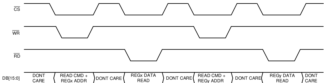
Figure 69. Parallel Interface Register Read
