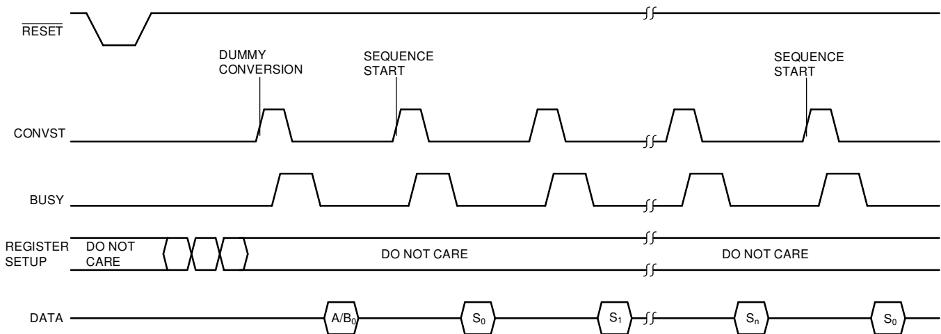
Figure 61. Software Mode Sequencer Configuration
