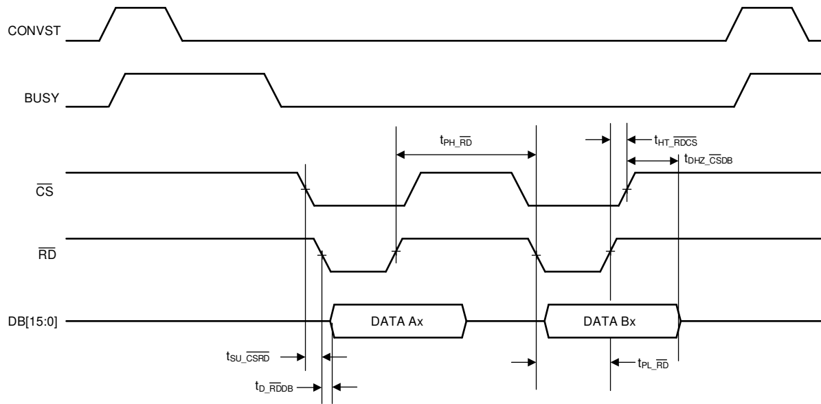
Figure 3. Parallel Read Timing Diagram
