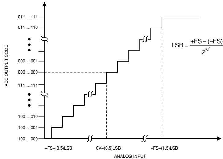
Figure 54. Transfer Characteristics
