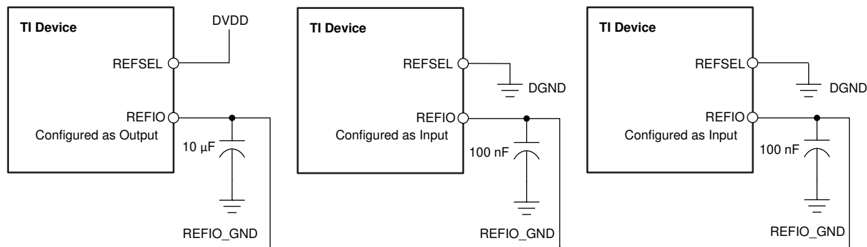
Figure 52. Multiple Devices Connected with an Internal Reference from One Device
