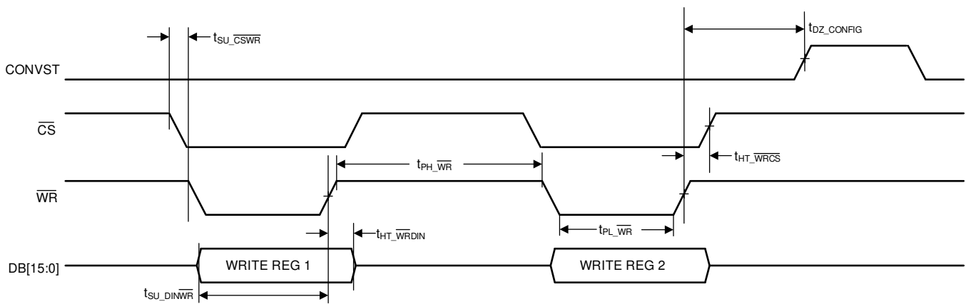
Figure 4. Parallel Write Timing Diagram
