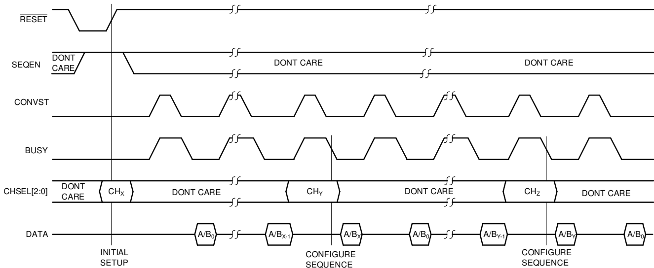
Figure 60. Hardware Mode Sequencer Configuration
