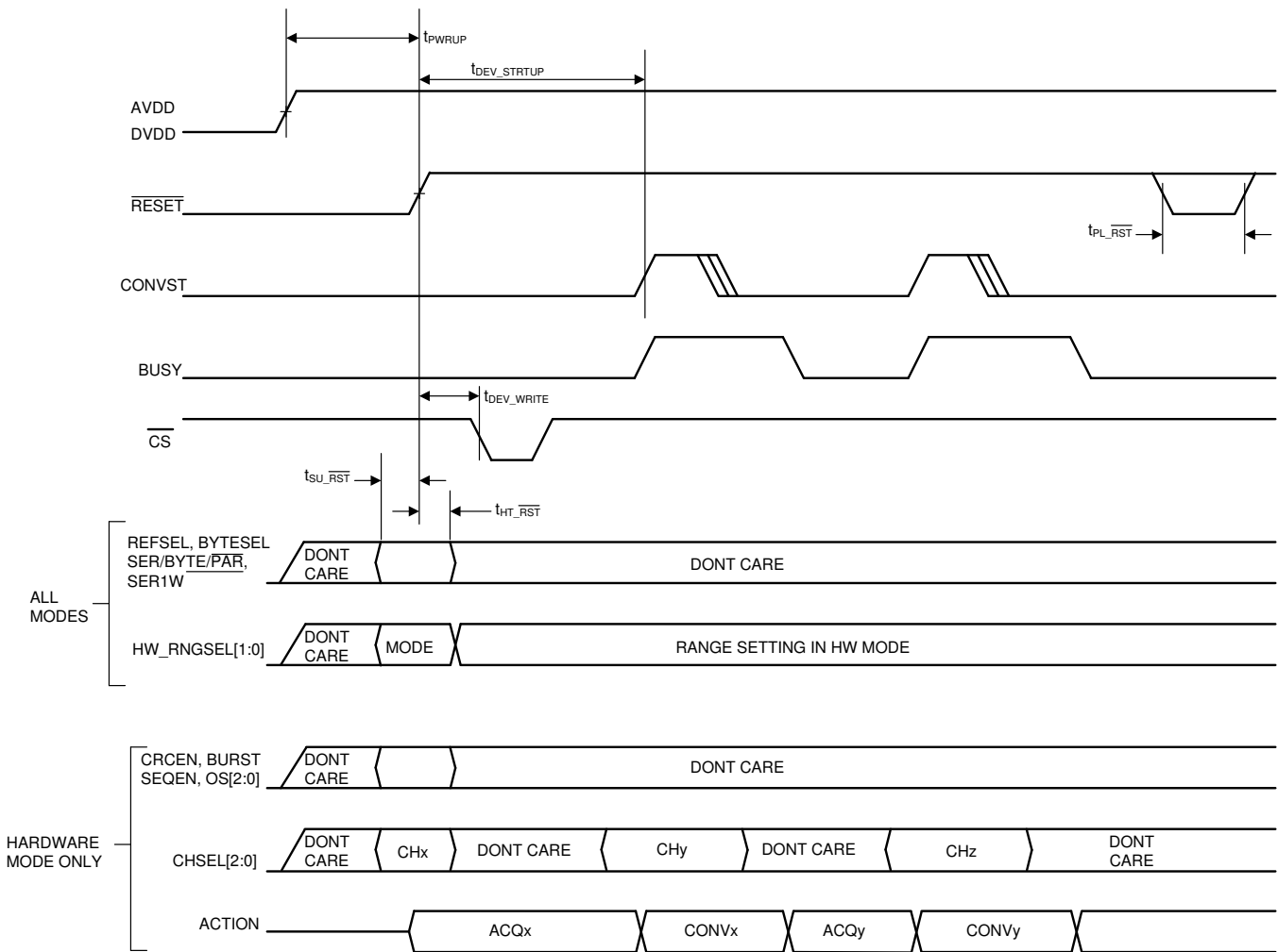
Figure 2. Reset Timing
