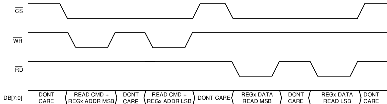
Figure 72. Parallel Byte Interface Register Read
