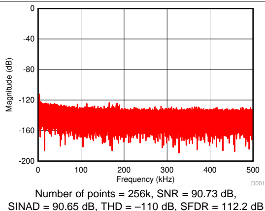
Figure 6. Typical FFT Plot ( \pm 10\text{ V} , Normal Mode, Filter Option 1)
