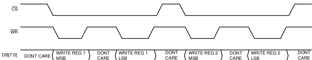
Figure 71. Parallel Byte Interface Register Write
