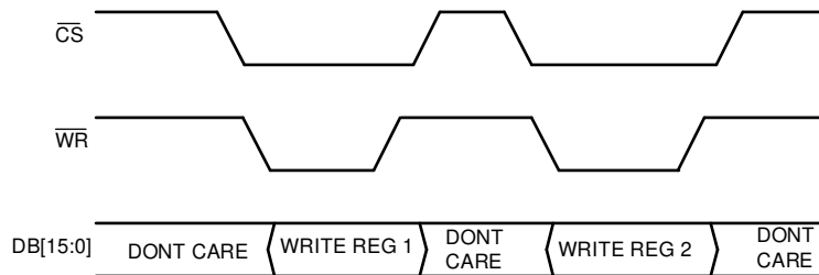
Figure 68. Parallel Interface Register Write
