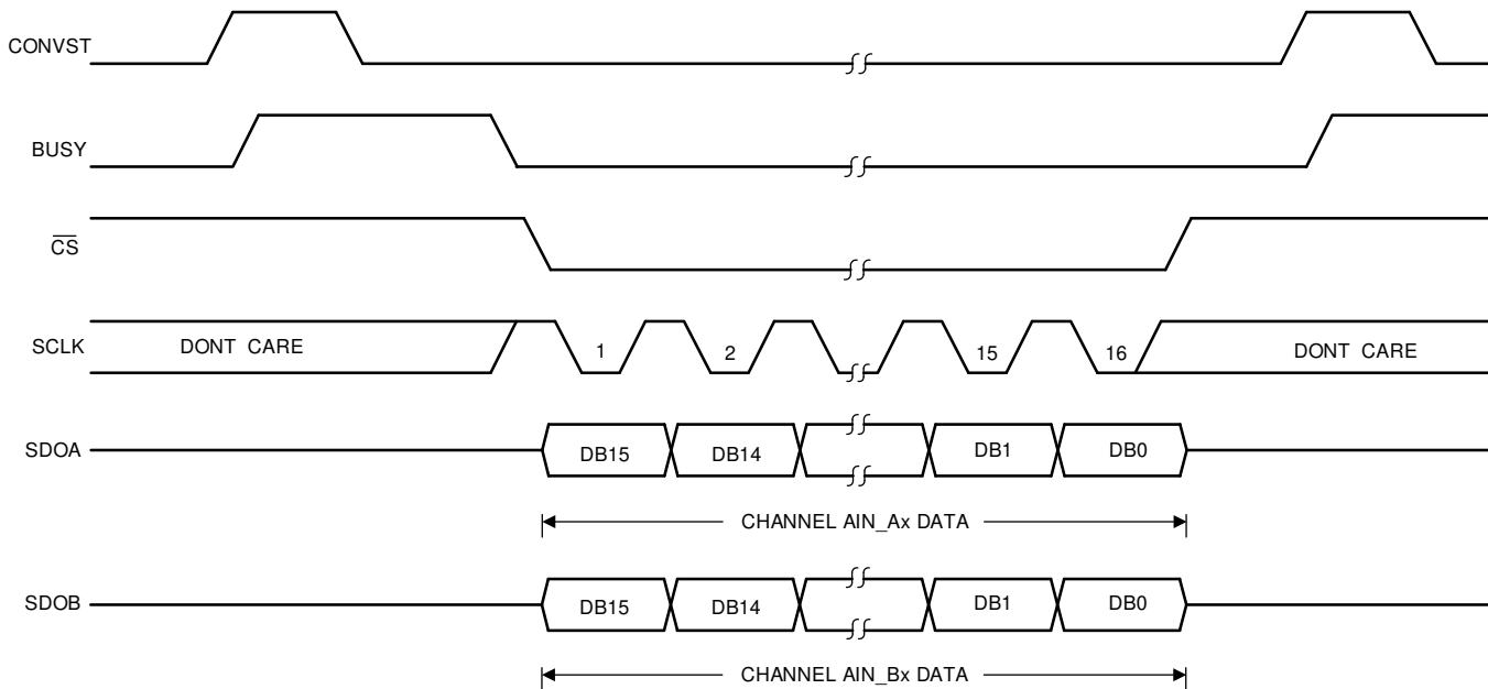
Figure 73. Serial Interface, 2-Wire Mode
