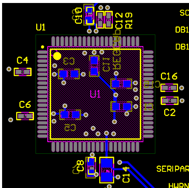
Figure 127. Bottom Layer Layout
