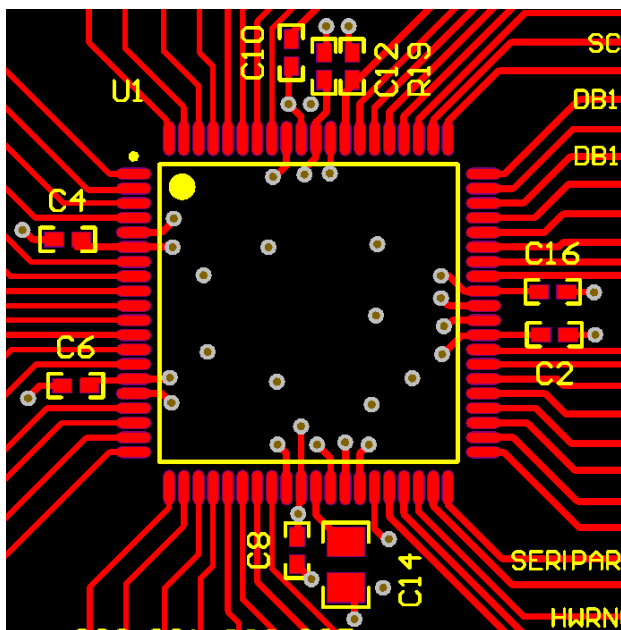
Figure 126. Top Layer Layout
