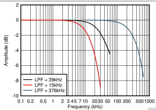
Figure 43. Frequency Response Across LPF Settings (±10 V)
