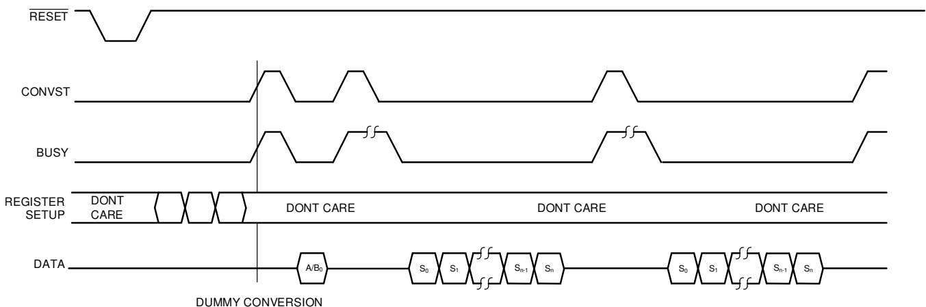
Figure 63. Burst Sequencer, Software Mode
