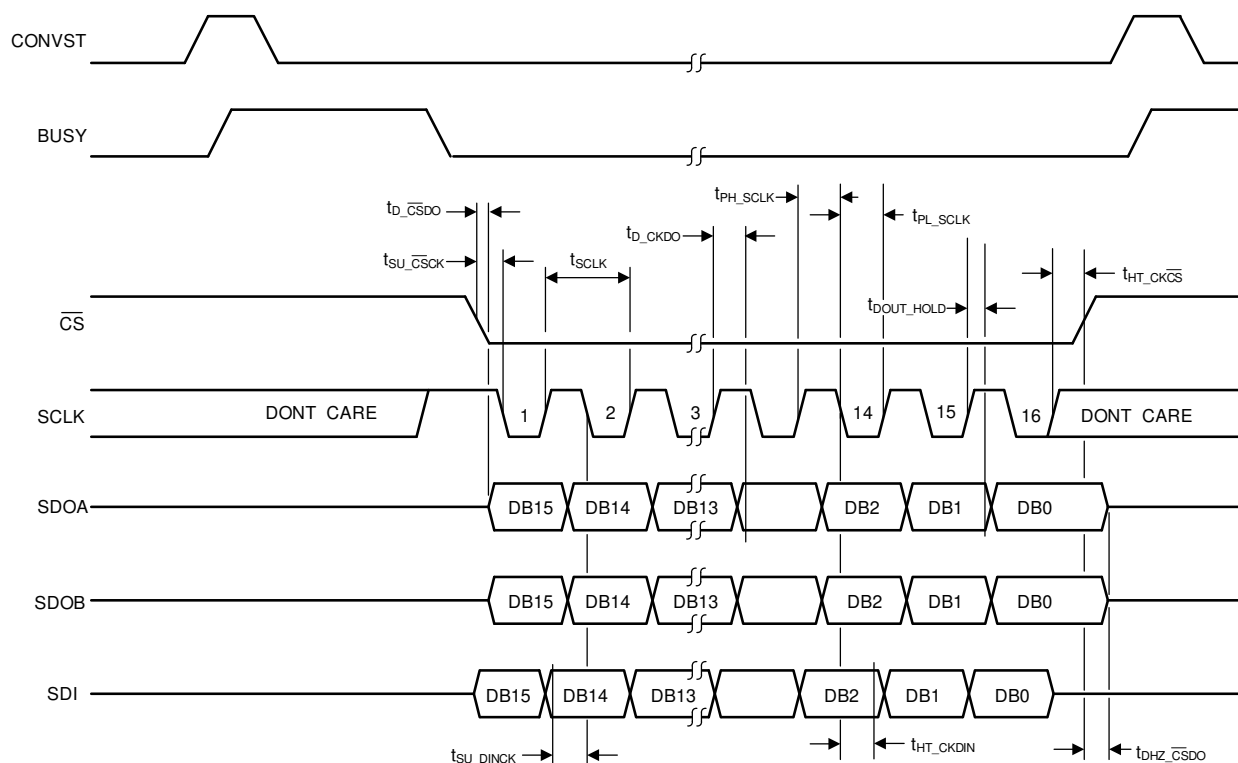
Figure 5. Serial Timing Diagram
