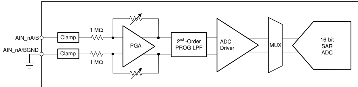
Figure 45. Front-End Circuit Schematic for the Selected Analog Input Channel
