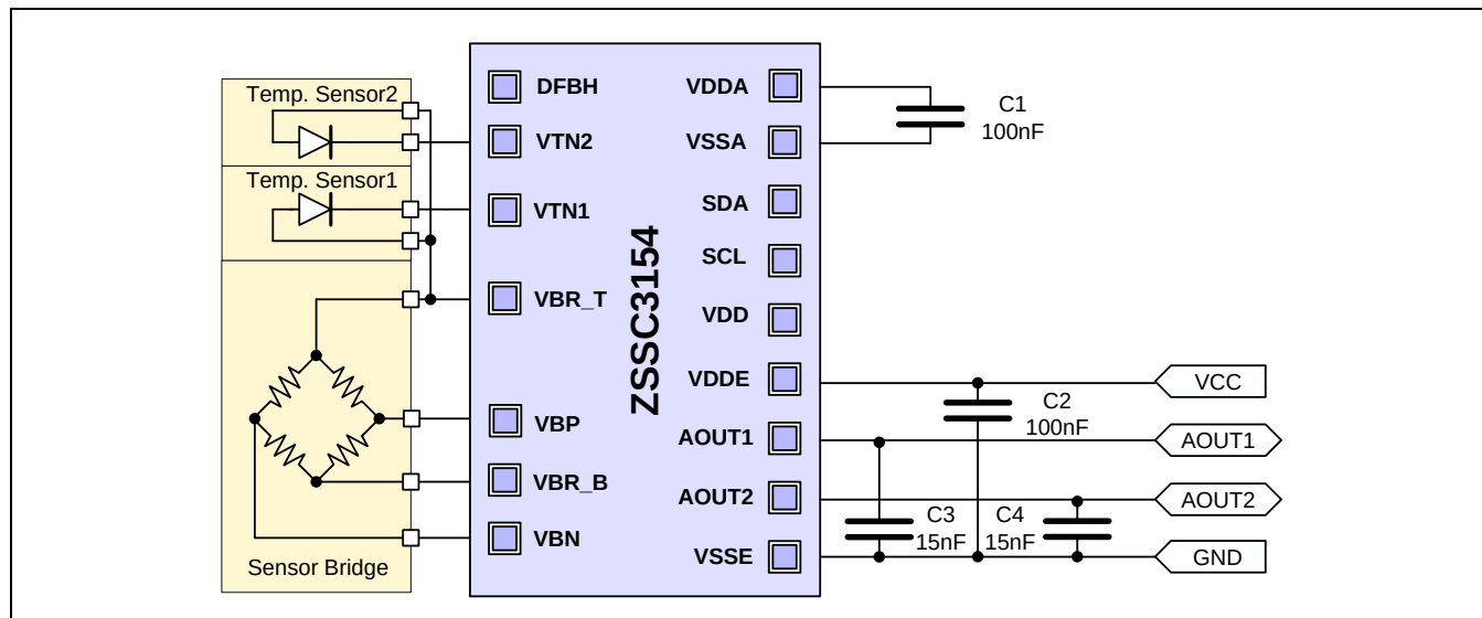
Figure 3.1 Application Circuit with Two Analog Outputs and Diagnostic Fault Band Level Low
