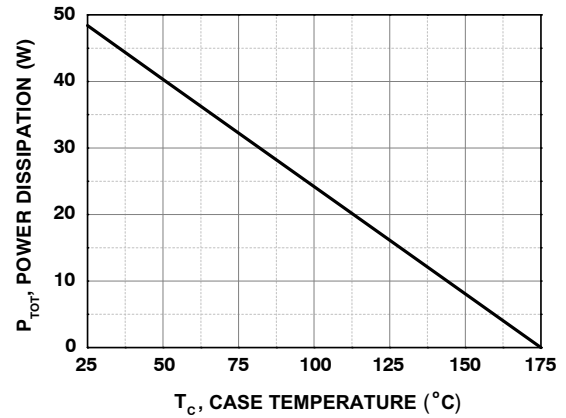
Figure 4. Power Derating
