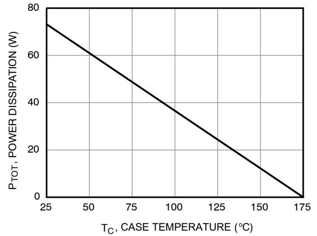
Figure 4. Power Derating
