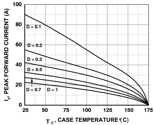
Figure 4. Current Derating
