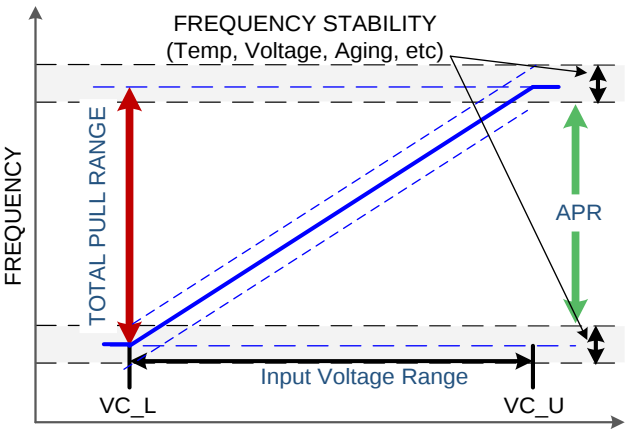
Figure 26. Typical SiTime VCTCXO FV Characteristic
