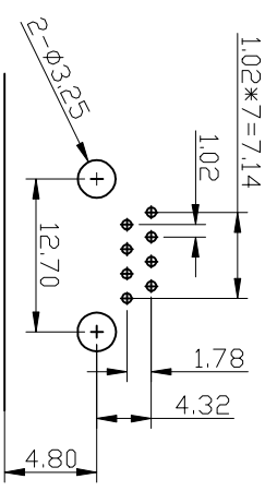
PC Board Layout Component Side Shown
