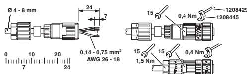
Functional drawing
