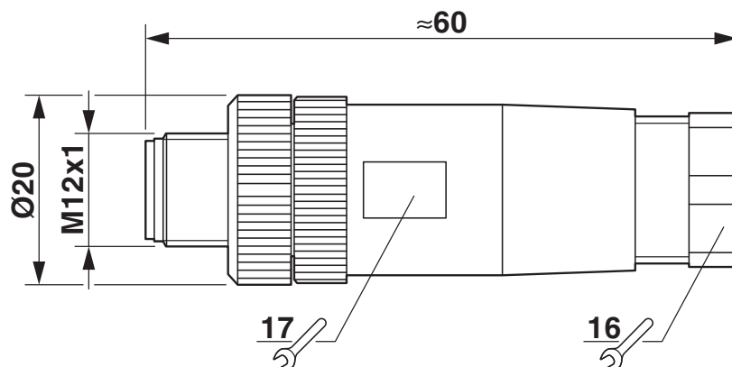
Dimensional drawing
