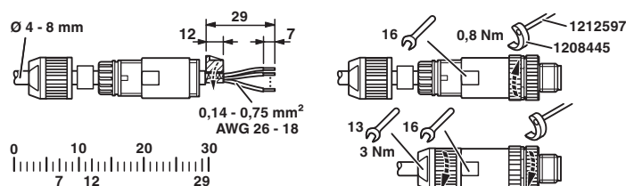
Functional drawing
