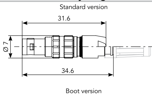
Breakaway Plug (FG)*
