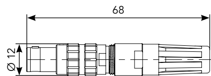
Straight Plug (FF)
