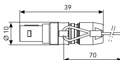
Straight Plug with Lanyard (FN) *
