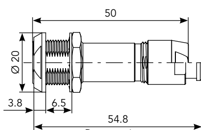
Rear Mount Cable (SA)*
