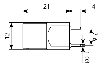
PCB Rear Mount with Mounting Pins (EZ)
