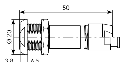
Rear Mount Cable (SA)*
