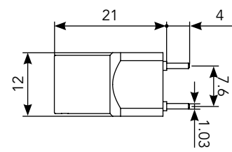
PCB Rear Mount with Mounting Pins (EZ)
