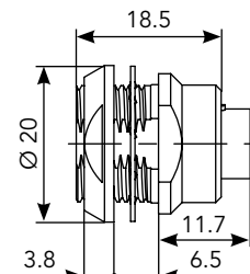
Rear Mount (EP)
