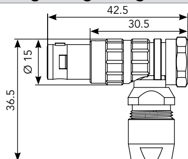
Right Angle Plug (FC)*
