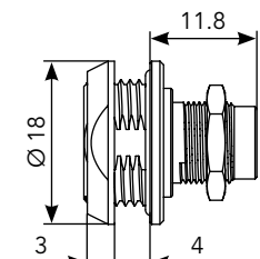
Rear Mount (HC)
