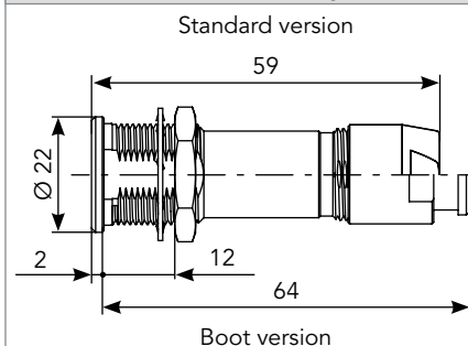
Front Mount Cable Receptacle (SR)*
