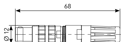
Straight Plug (FF)
