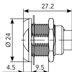
Double Nut (EA)
