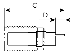
Female Insulator
