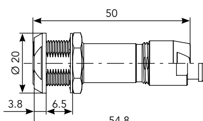
Rear Mount Cable (SA)*
