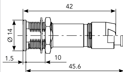
Front Mount Cable (SR)*
