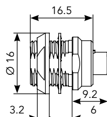
Rear Mount (EP)
