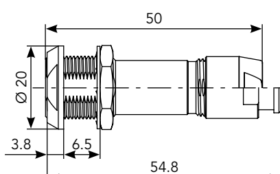
Rear Mount Cable (SA)*
