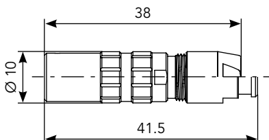
In Line Cable Receptacle (PC)*
