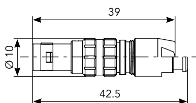
Straight Plug (FD)*
