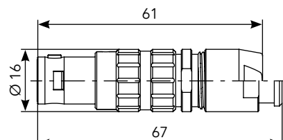
Straight Plug (FD)*
