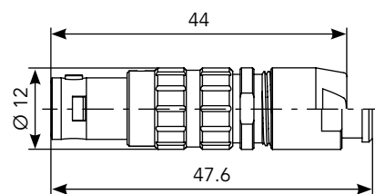
Straight Plug (FD)*
