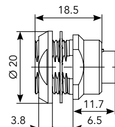
Rear Mount (EP)
