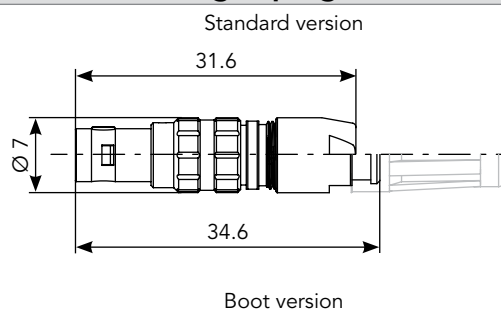
Straight plug (FD)*
