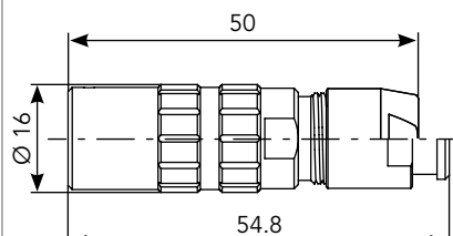
In Line Cable (PC)*
