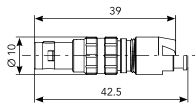
Straight Plug (FD)*
