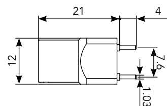
PCB Rear Mount with Mounting Pins (EZ)
