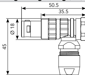
Right Angle Plug (FC)*
