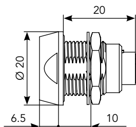
Double Nut (EC)
