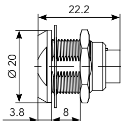
Double Nut (EA)
