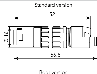
Straight Plug (FH)*
