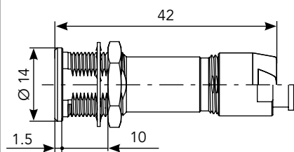
Front Mount Cable (SR)*
