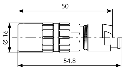
In Line Cable (PC)*
