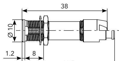
Front Mount Cable Receptacle (SR)*
