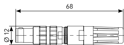
Straight Plug (FF)
