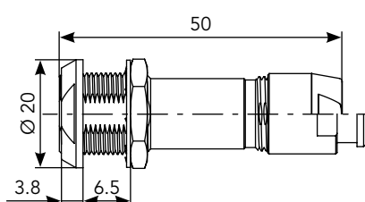
Rear Mount Cable (SA)*
