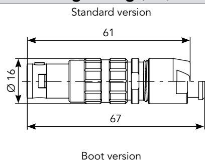
Straight Plug (FD)*
