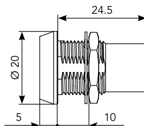
Front Mount Extended (HH)
