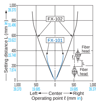
FT-S31W Thru-beam type
