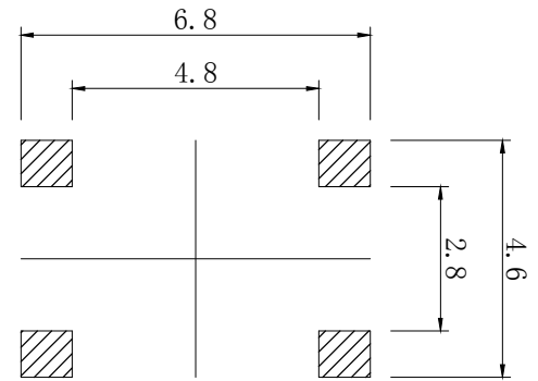
PCB.WELDING DRAWING
