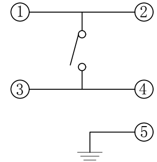
CIRCUIT DIAGRAM
