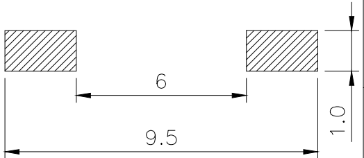
PCB WELDING DRAWING
