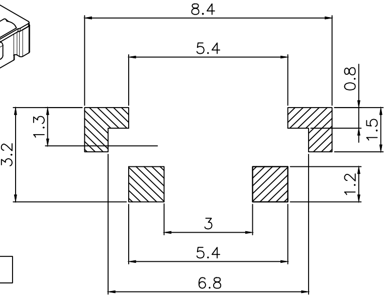
PCB. WELDING DRAWING
