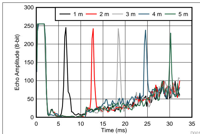
图 139. Long Range ISO-Pole Measurements Using Transformer Drive
