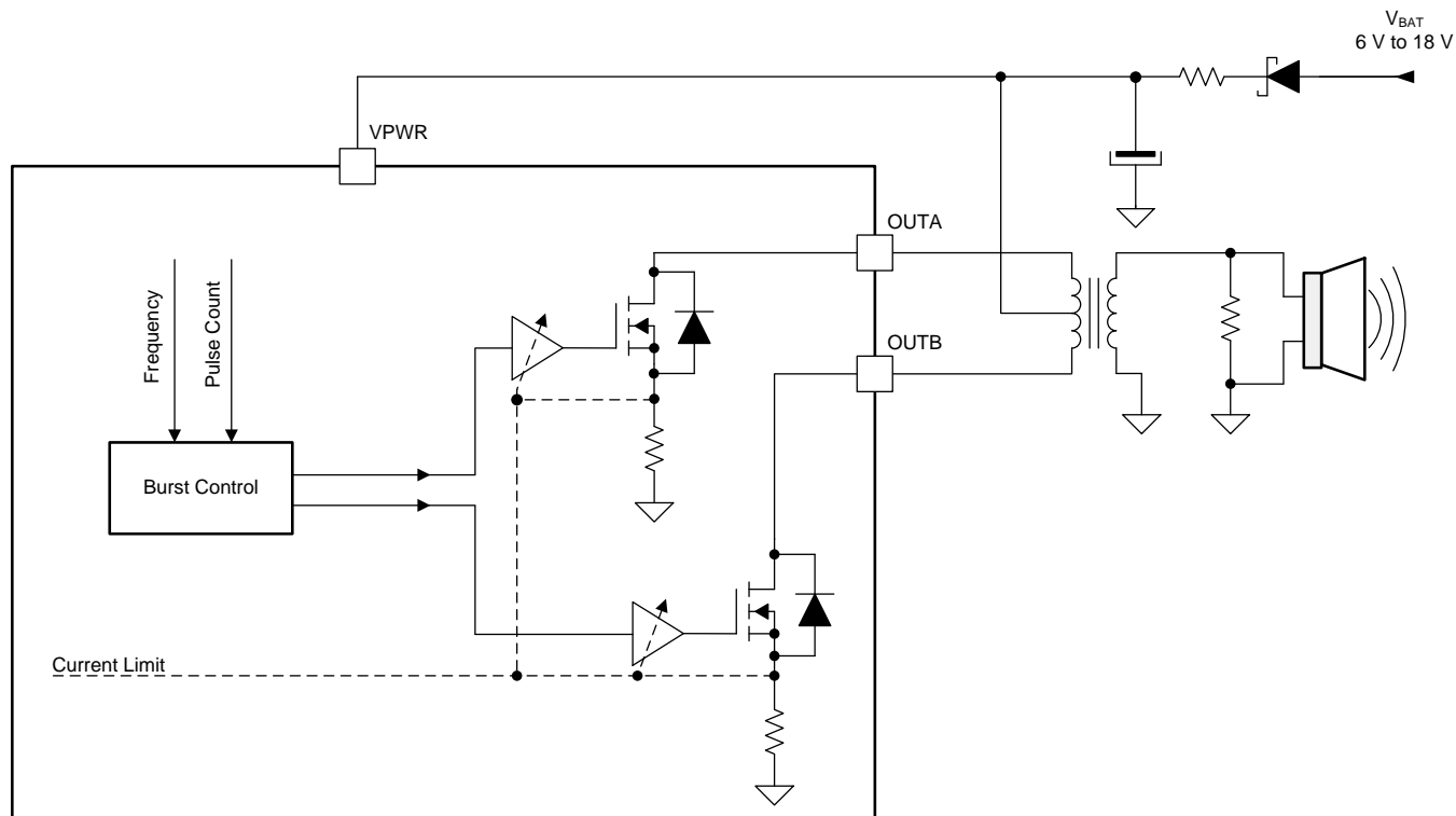
图 3. Echo Generation Block Diagram
