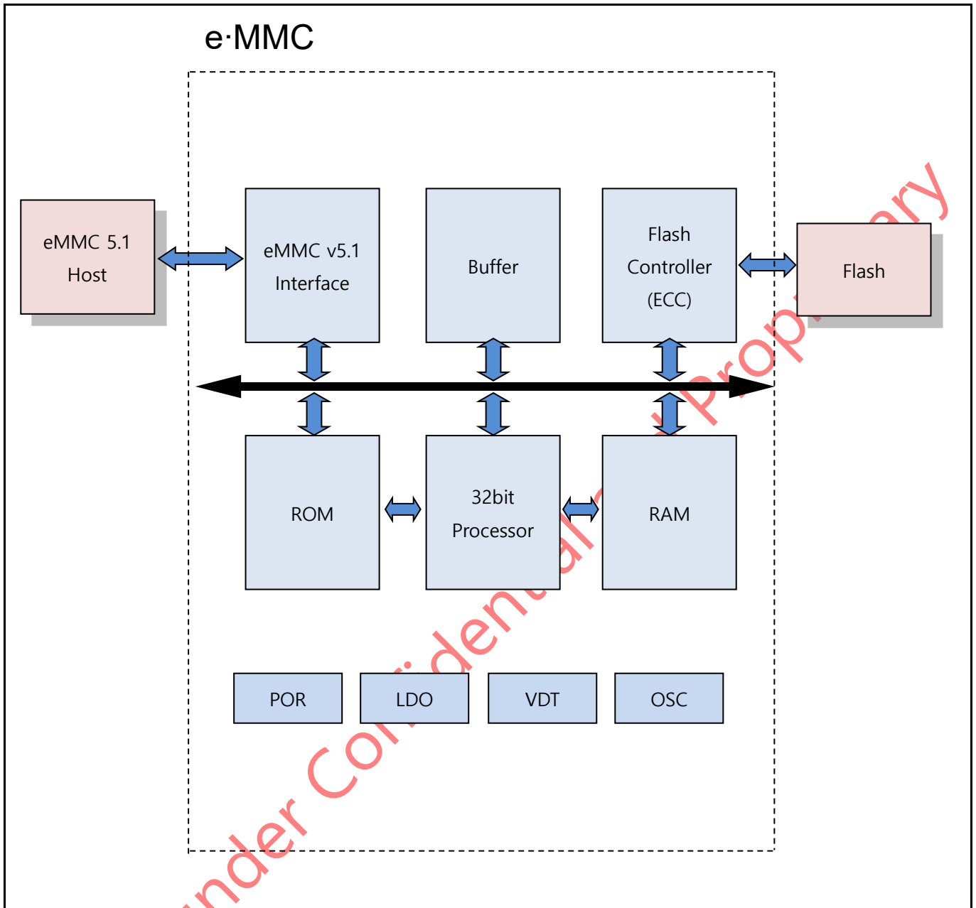
Figure 1 - e-MMC Block Diagram
