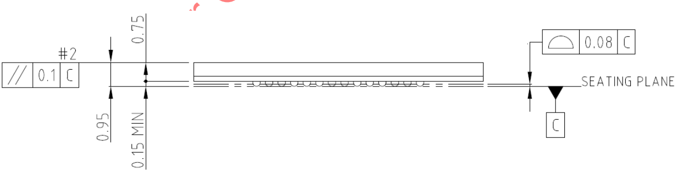
Figure 5 – 11.5 x 13.0 x 1.0mm Bottom & side View
