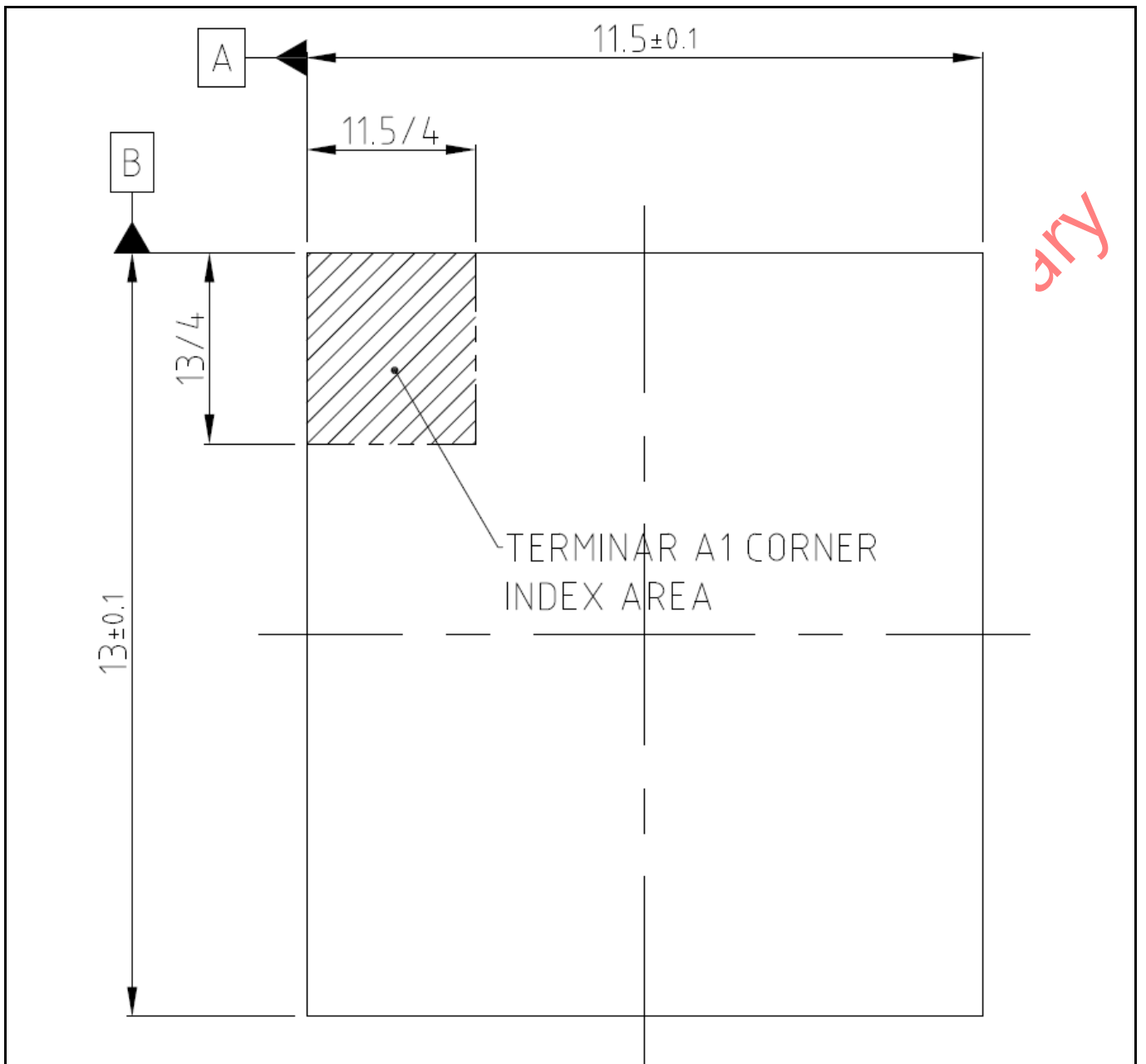
Figure 4 – 11.5 x 13.0 x 1.0mm Top View
