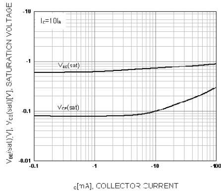
Figure 3. Base-Emitter Saturation Voltage Collector-Emmitter Saturation Voltage
