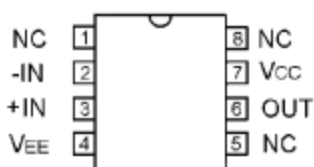
(D08S2·顶视图)
