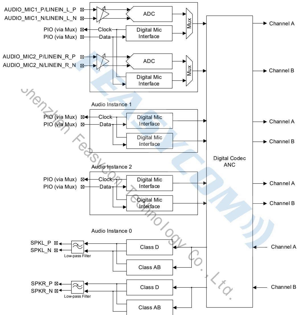
Figure 8: FSC-BT1026x analog audio and microphone interfaces
