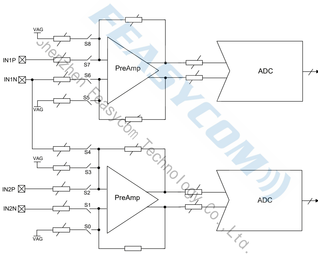
Figure 9:FSC-BT1026x high-quality ADC input switch configuration
