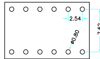
Recommended P. C. B Layout (±0.05)
