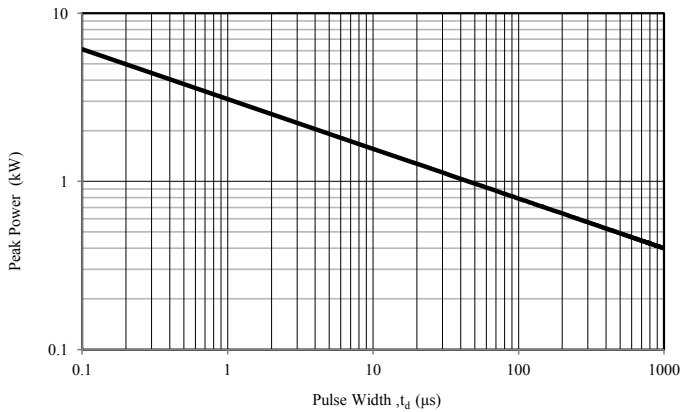
Fig. 5 - Steady State Power Derating Curve
