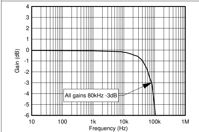
图 7-3. Sensitivity vs. Frequency, All Gains Normalized to 1 Hz
