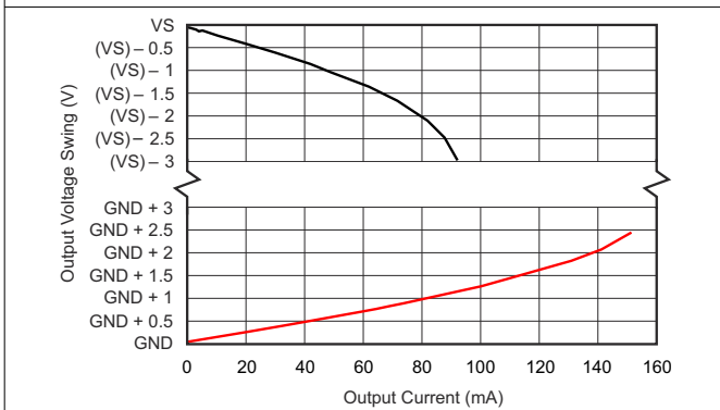
图 7-5. Output Swing vs. Output Current
