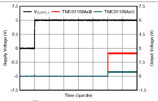
图 7-12. Startup Transient Response
