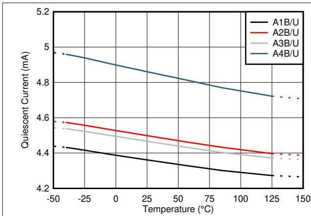
图 7-7. Quiescent Current vs. Temperature
