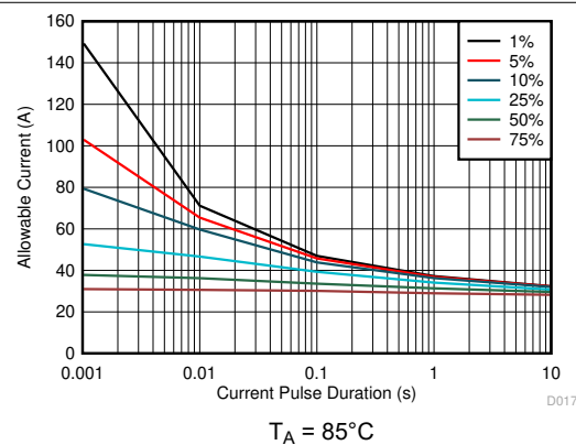
图 8-7. Maximum Repetitive Pulsed Current vs Pulse Duration
