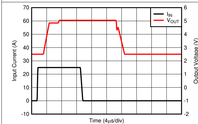
图 7-11. Current Overload Response
