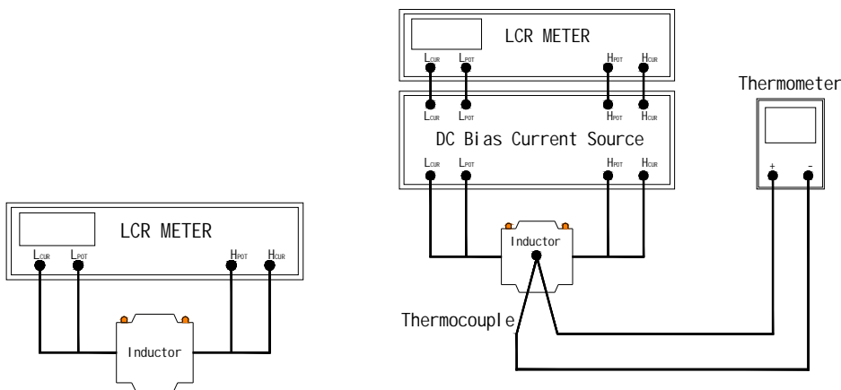
Is & RDC test schematic diagram
