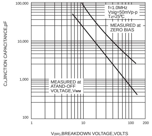
FIG. 4-TYPICAL JUNCTIONAL CAPACITANCE
