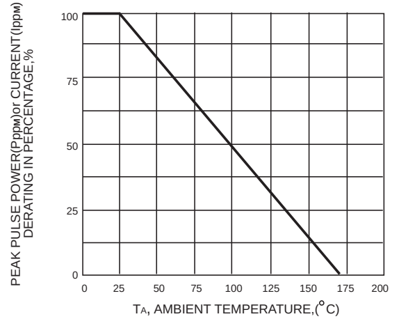
FIG. 2-PULSE DERATING CURVE
