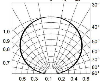
Fig.6-Radiation Diagram Ta=25°C
