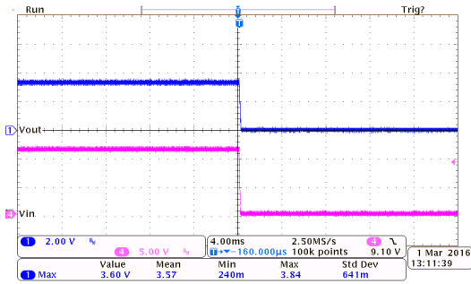
掉电响应: HT7333-7 ( I_{OUT}=250mA , T_{FALL}=0.1ms )
