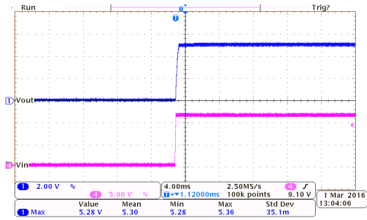
上电响应: HT7350-7 ( I_{OUT}=250mA , T_{RISE}=0.1ms )
