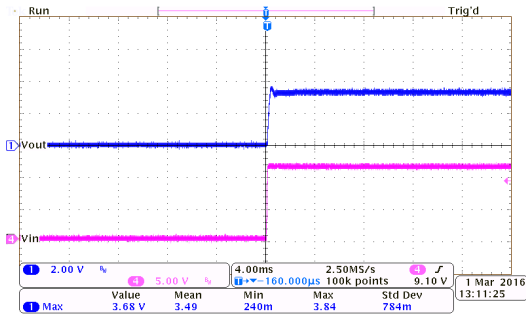
上电响应: HT7333-7 ( I_{OUT}=250mA , T_{RISE}=0.1ms )
