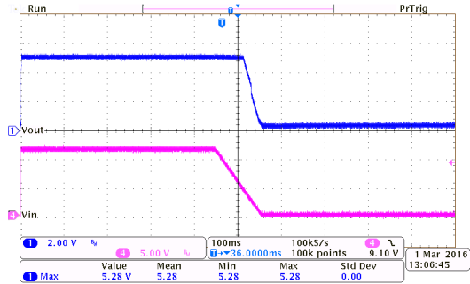
掉电响应: HT7350-7 ( I_{OUT}=0mA , T_{FALL}=100ms )
