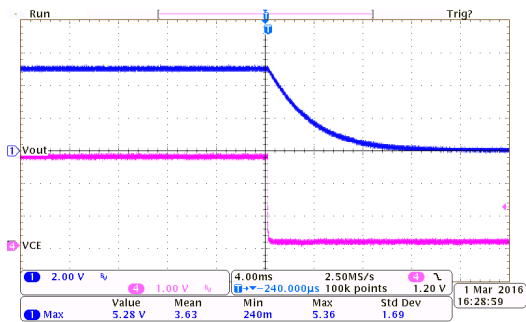
掉电响应: HT7350-7 ( I_{OUT}=0mA, V_{CE}=2.7V to 0V)
