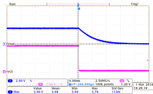
掉电响应: HT7333-7 ( I_{OUT}=0mA, V_{CE}=2.7V to 0V)
