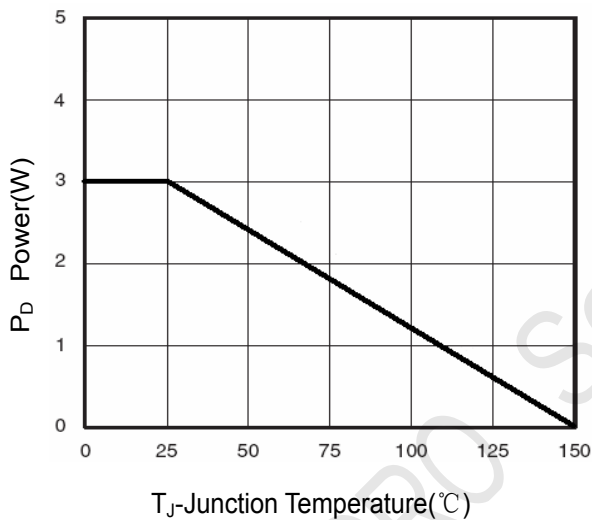
Figure 3 Power Dissipation
