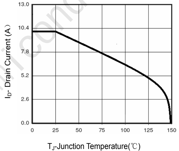
Figure 4 Drain Current
