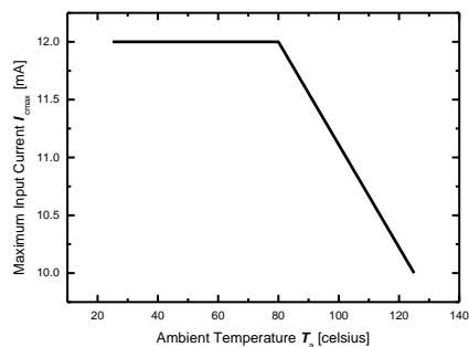
Figure 1. Maximum input current I_{cmax}
