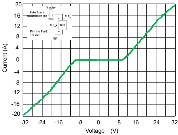
Fig 3. TLP Measurement
