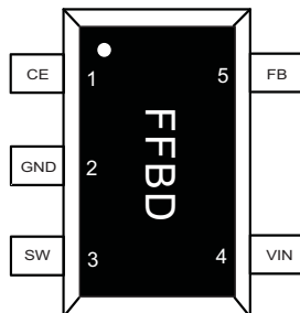
(SOT23-5L)
