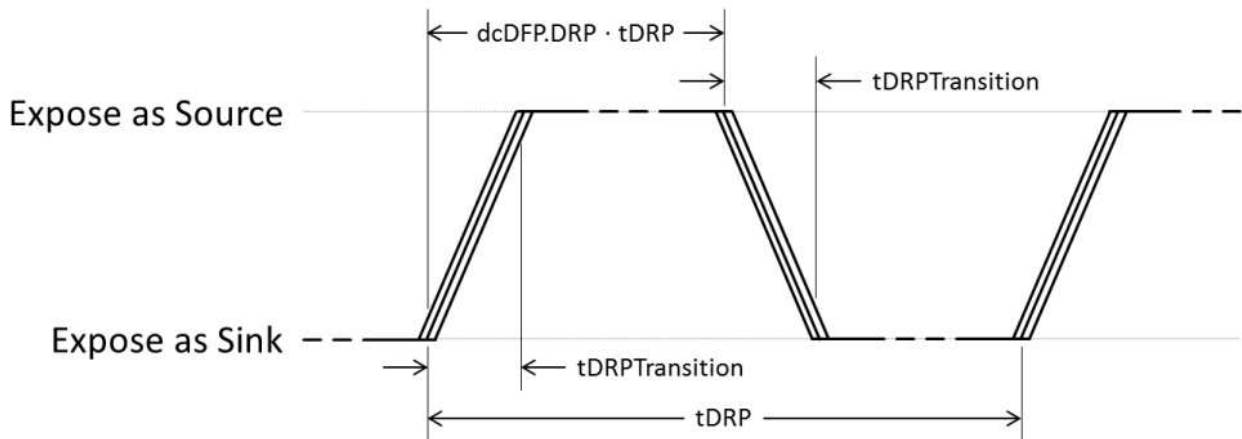
Figure 4-36 DRP Timing
