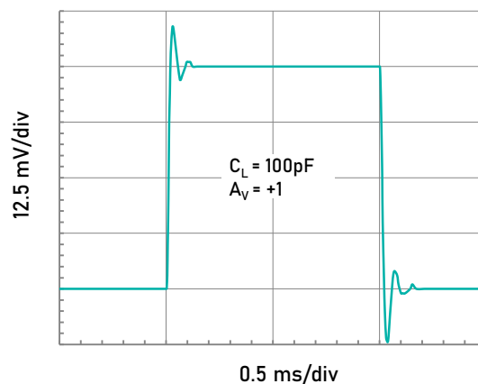
Small Signal Step Response (50mV Step).
