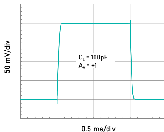
Small Signal Step Response (200mV Step).
