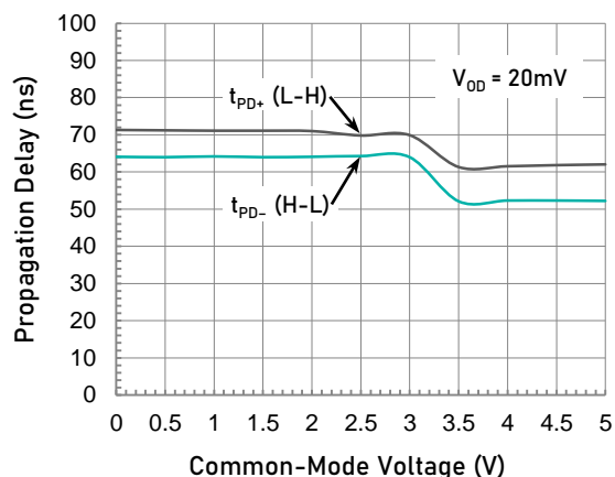
Propagation Delay vs. Input Common-Mode
