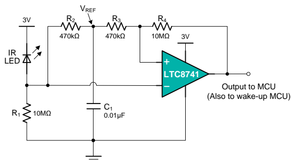
Figure 5. IR Receiver AFE Using LTC8741
