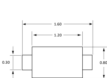
Package Dimensions
