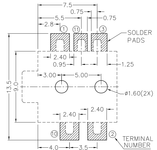
RECOMMENDED SOLDER PAD LAYOUT
